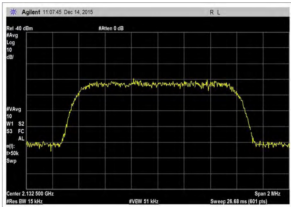
7.10_OBW_DL_2110-2155MHz_CDMA
