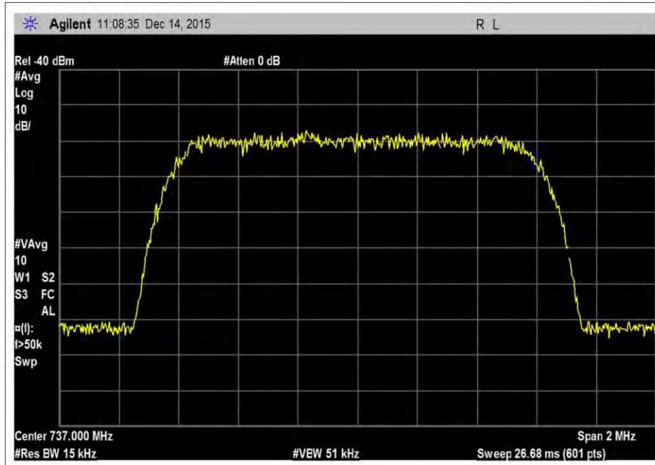
7.10_OBW_DL_728-746MHz_CDMA
