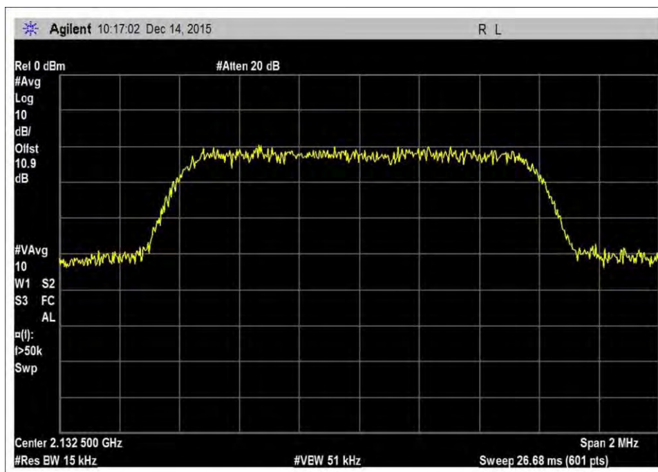
7.10_OBW_DL_2110-2155MHz_CDMA
