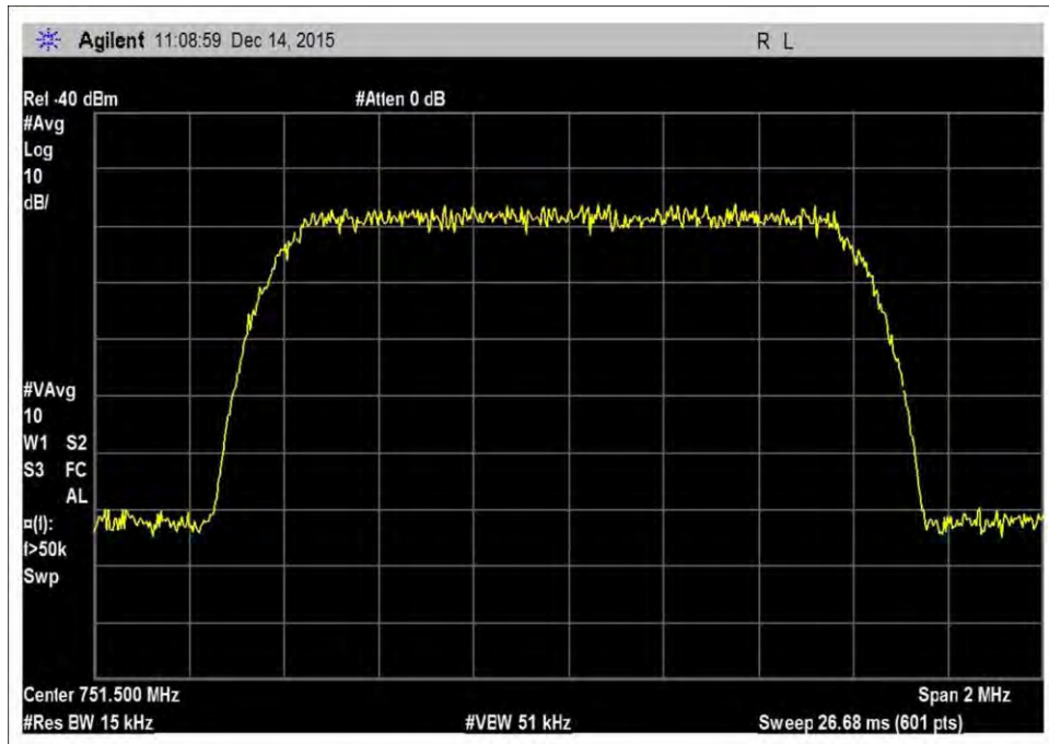
7.10_OBW_DL_746-757MHz_CDMA
