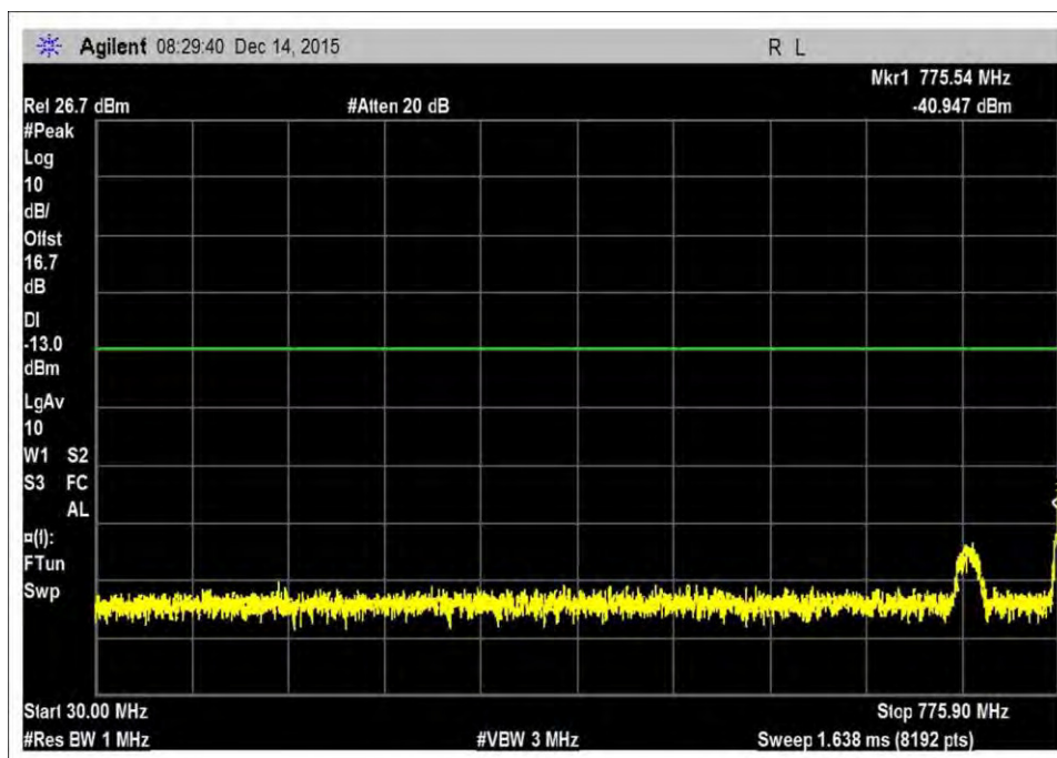
UL_776-787L
