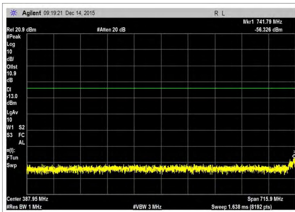
DL_746-757L
