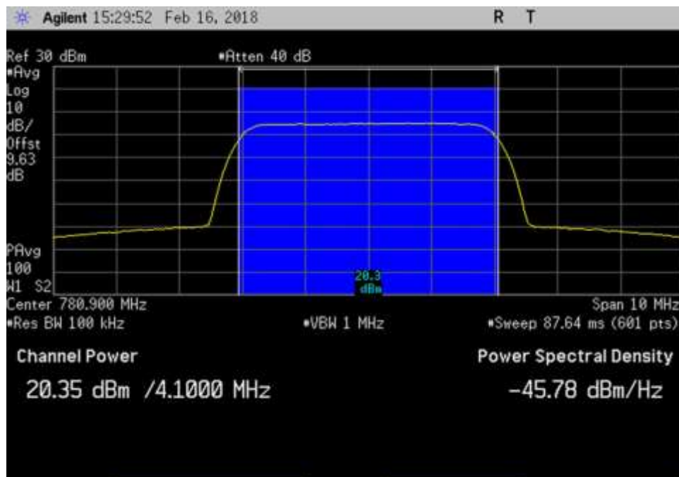
UL_776-787_AWGN_Max_780.9MHz
