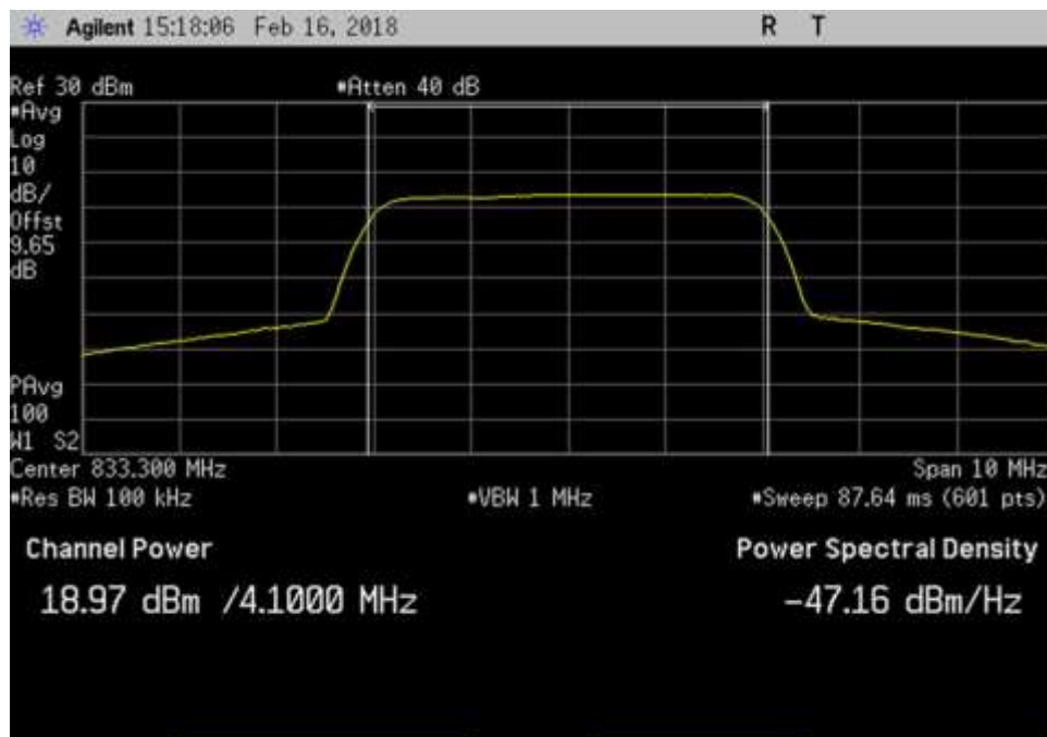
UL_824-849_AWGN_Max_ 833.3MHz
