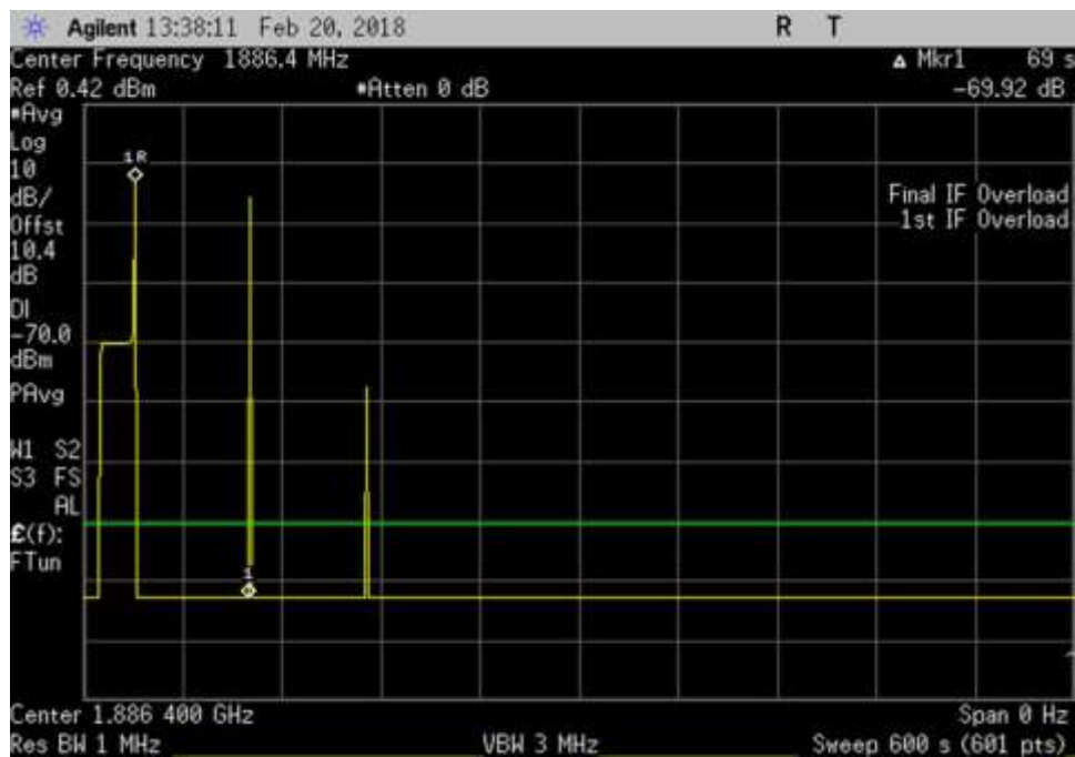
UL_1850-1915_600sec_1886.4MHz
