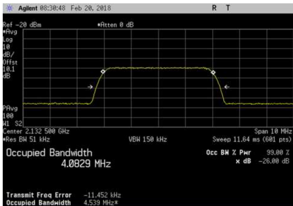
DL_2110-2155_AWGN_ 2132.5MHz
