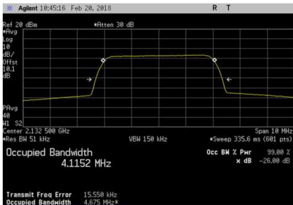
DL_2110-2155_AWGN_ 2132.5MHz
