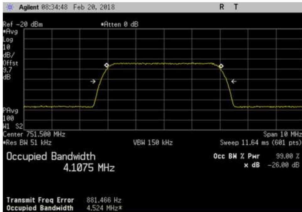
DL_746-757_AWGN_751.5MHz
