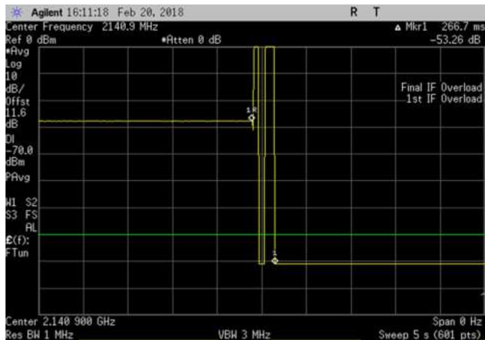
DL_2110-2155_ 2140.9MHz_Time
