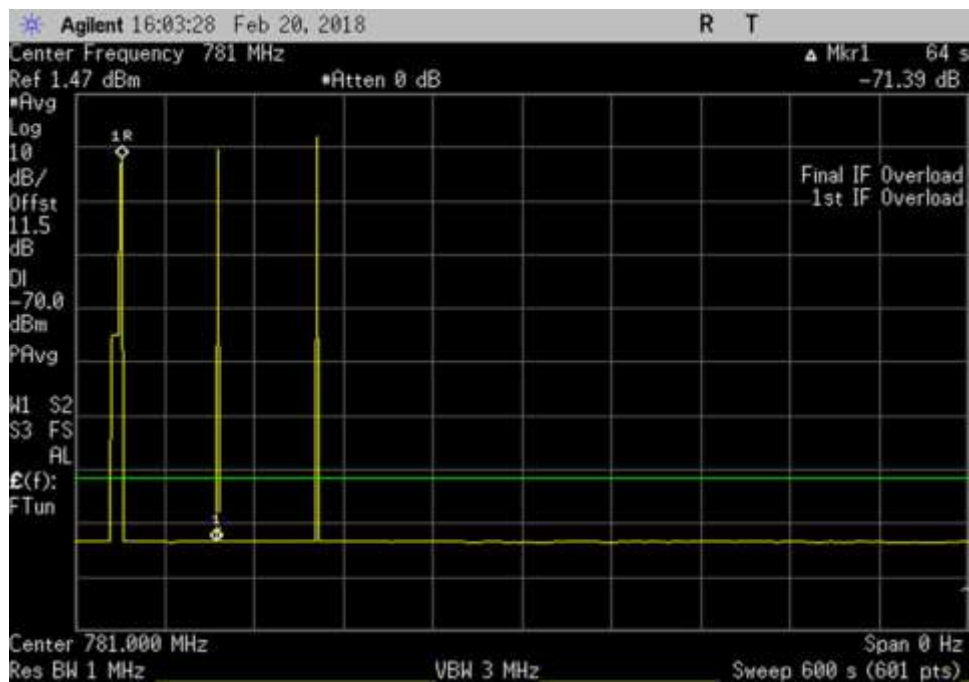
UL_776-787_600sec_781MHz
