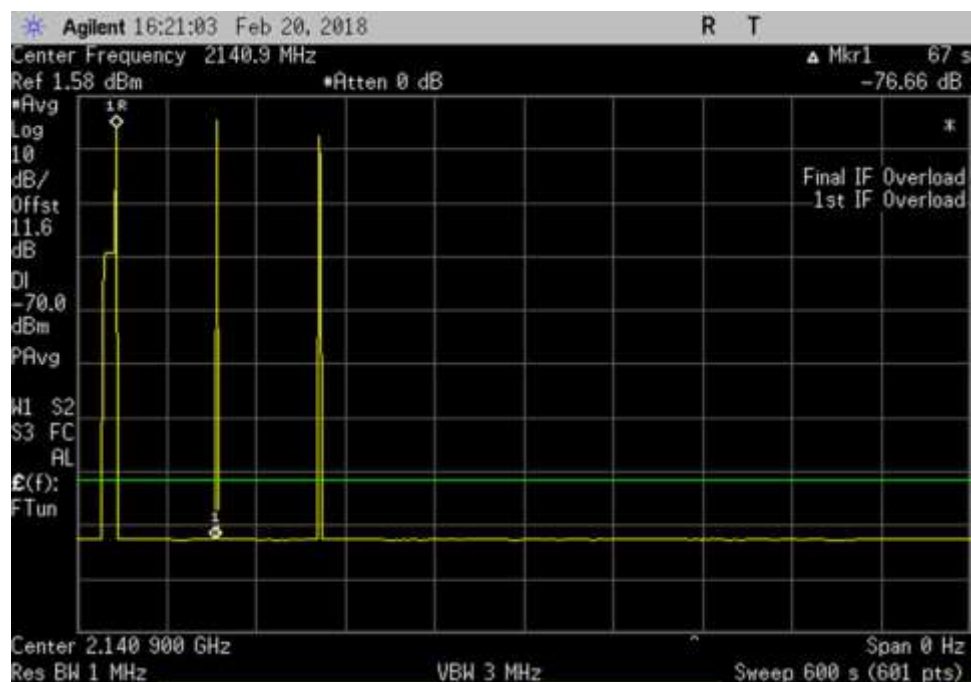
DL_2110-2155_600sec_ 2140.9MHz
