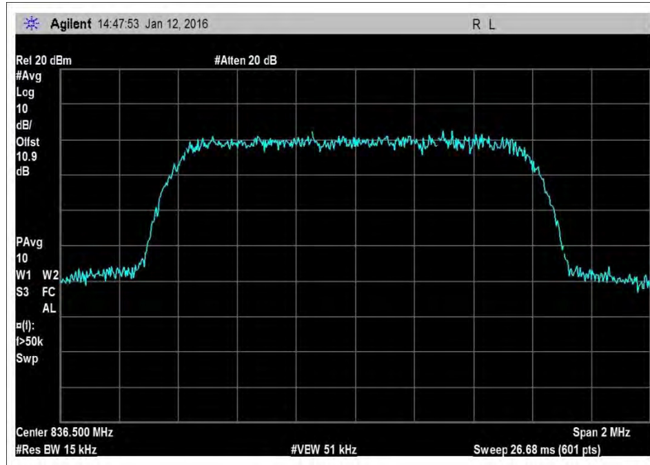
7.10_OBW_UL_824-849MHz_CDMA
