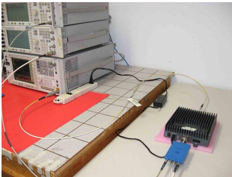
7.4 Test Setup
