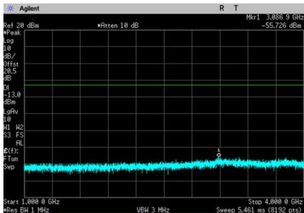
CSE_UL_788-798_1000-4000MHz_LC
