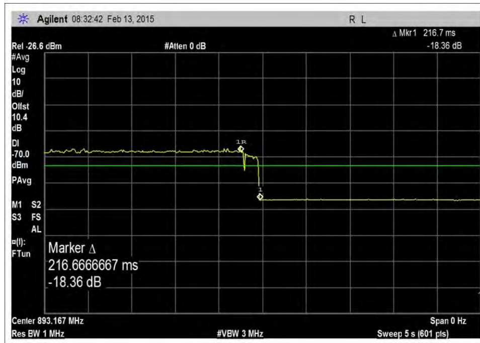
DL_869-894MHz_a-g_timing
