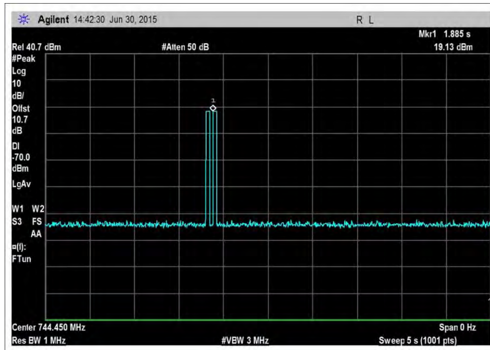
DL_728-746MHz-Pk
