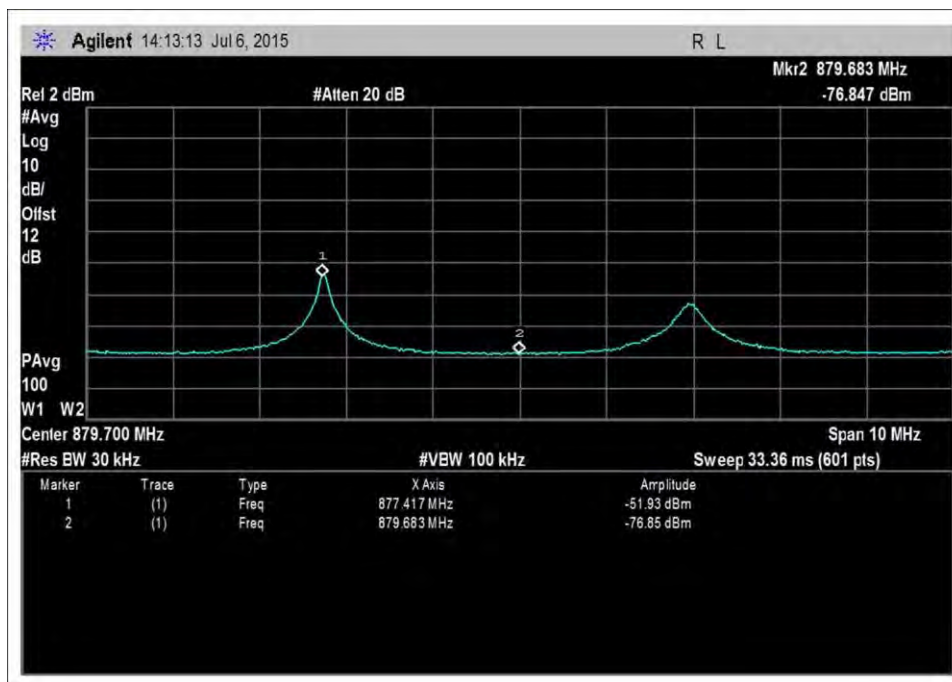
DL_869-894MHz-AWGNL+1
