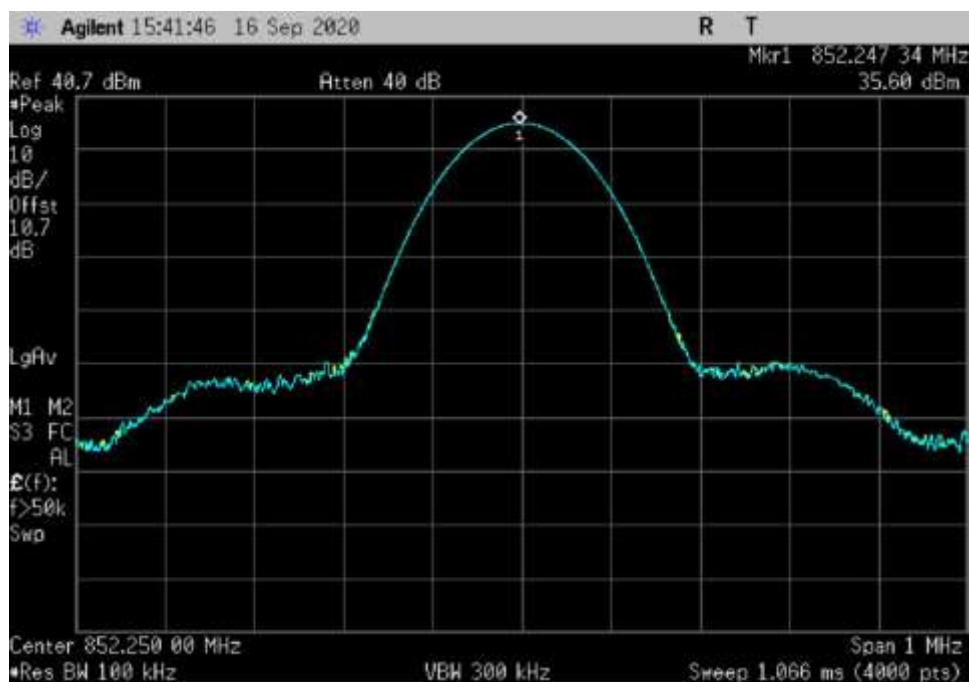
DL_851-854-CW-AGC+3_ 852.25MHz
