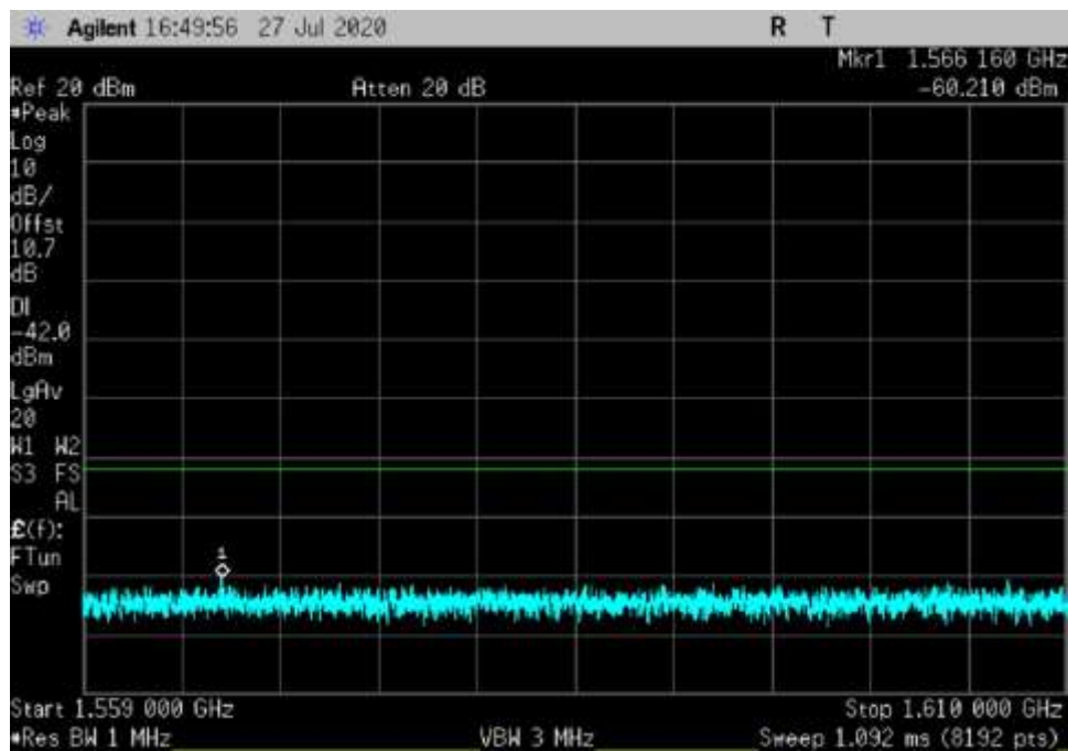
DL_769-775_1559-1610MHz_MC
