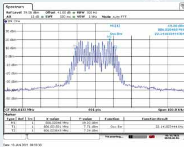
Low Frequency: 806.0125MHz, Output occupied BW(AGC)
