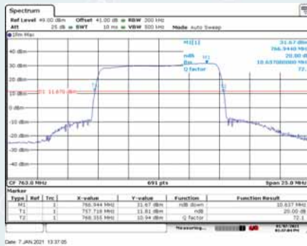
Downlink: 758MHz~768MHz
