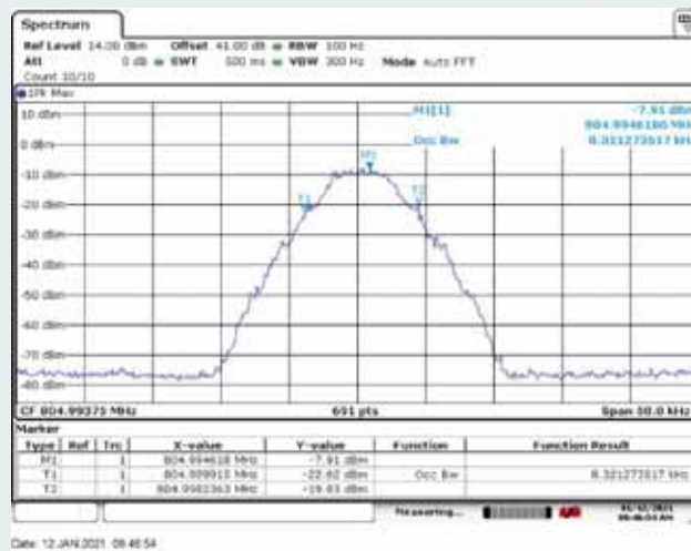
High Frequency: 804.99375MHz, Input occupied BW
