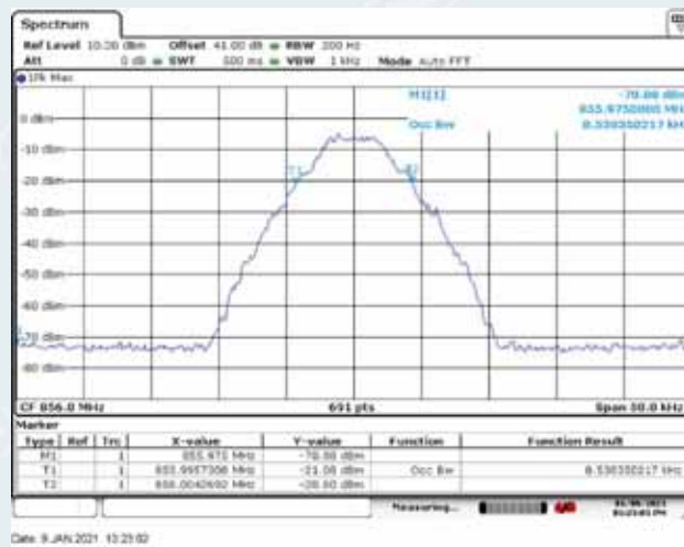
Downlink Frequency: 856.0MHz
