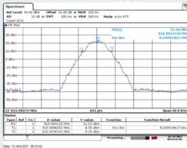
High Frequency: 815.99375MHz, Output occupied BW(AGC)
