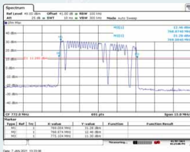
Downlink: 769MHz~775MHz
