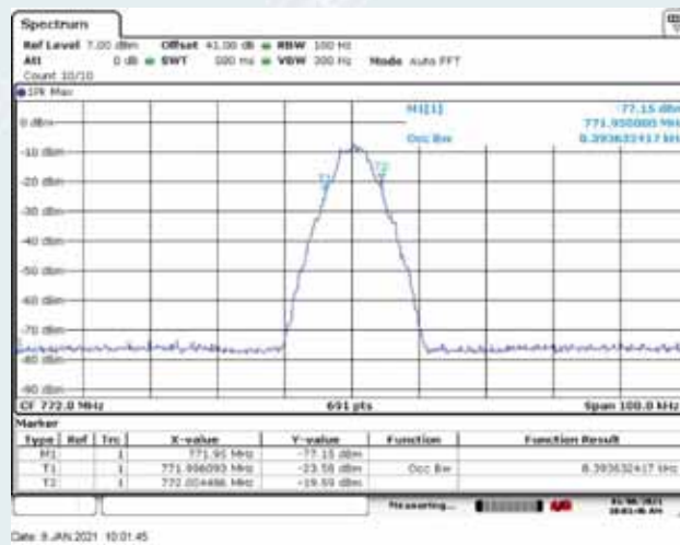
Downlink Frequency: 772.0MHz
