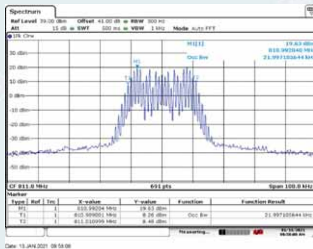
Middle Frequency: 811.0MHz, Output occupied BW(AGC)
