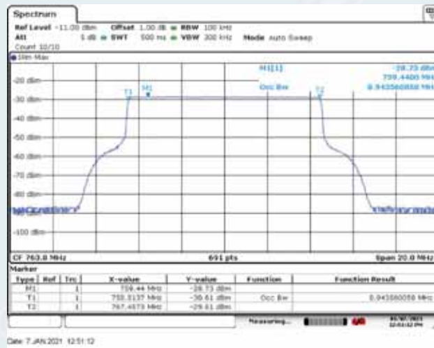
Downlink Frequency: 763MHz
