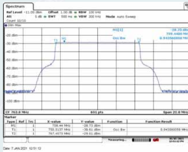
Frequency: 763.0MHz, Input occupied BW
