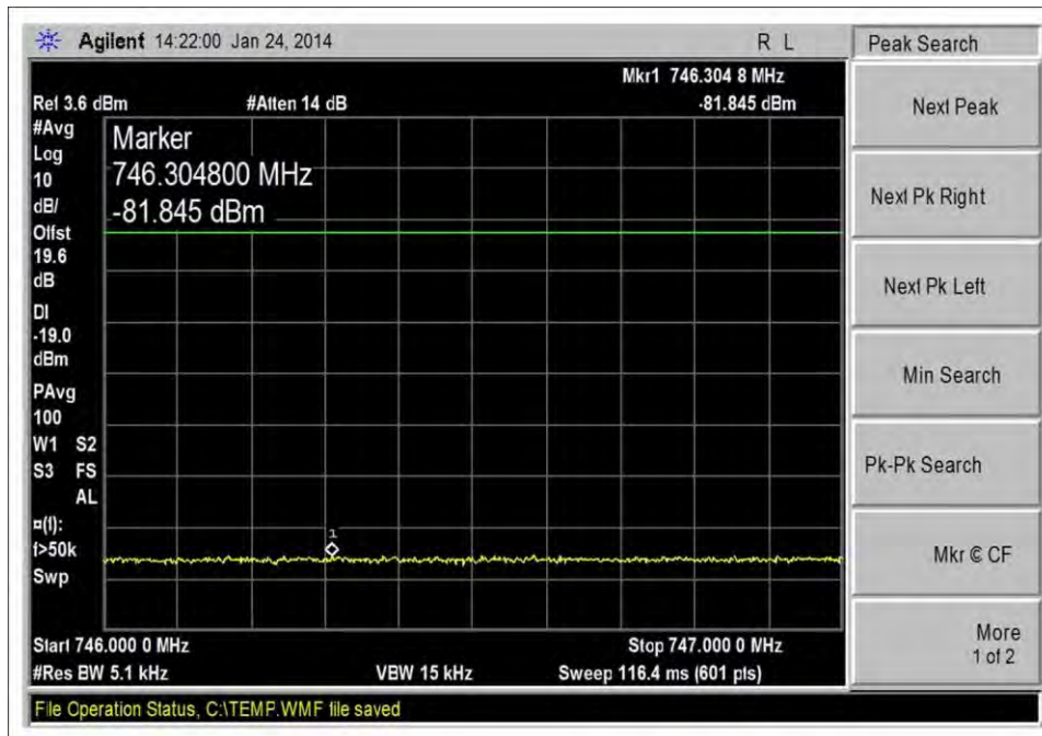
DL_728-746MHz_Hi CH_GSM_-20dbm
