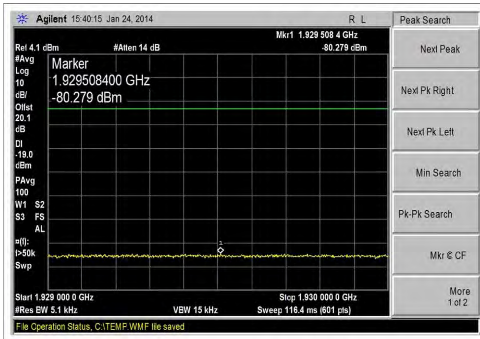
DL_1930-1990MHz_Low CH_GSM_-20dbm
