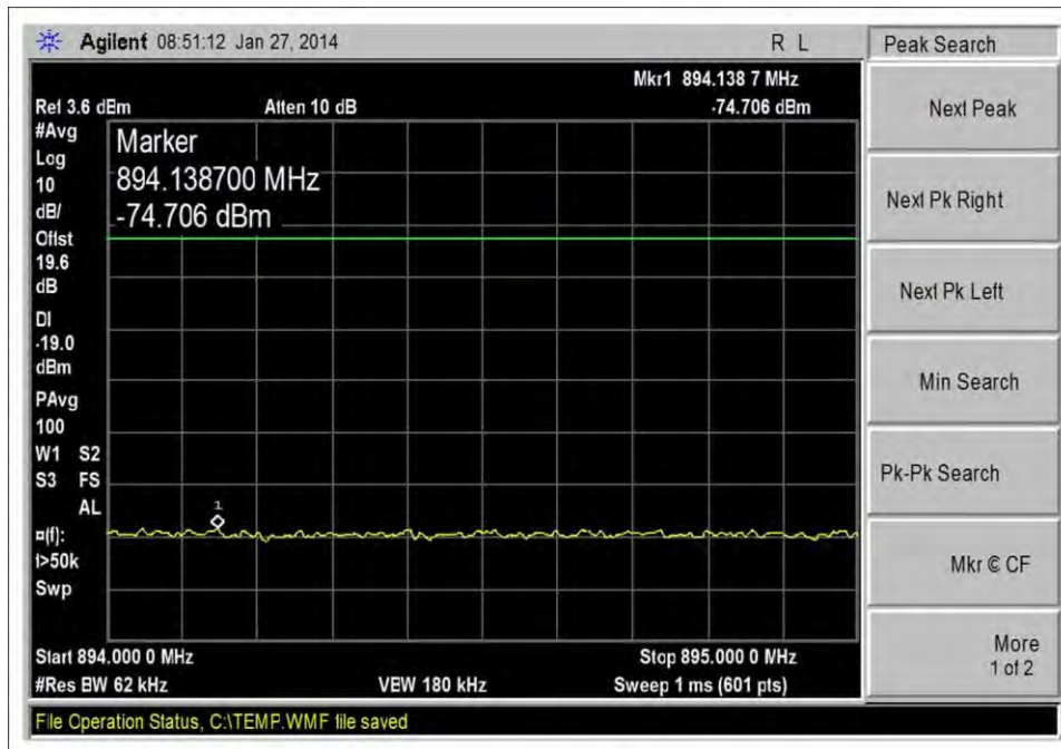
DL_869-894MHz_Hi CH_LTE_-20dbm
