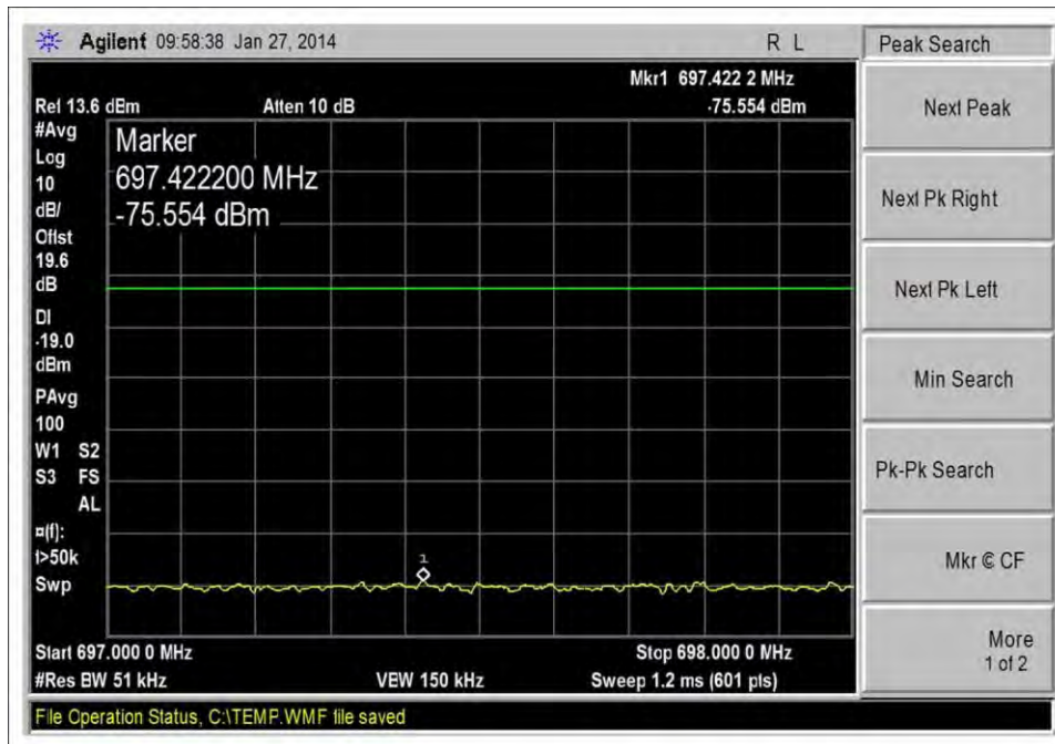
UL_698-716MHz_Low CH_CDMA_10dbm
