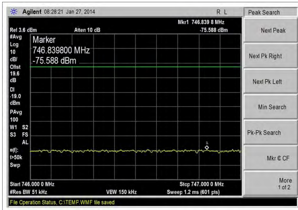
DL_728-746MHz_Hi CH_CDMA_-20dbm
