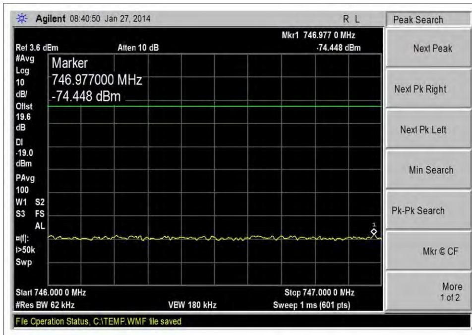
DL_728-746MHz_Hi CH_LTE_-20dbm
