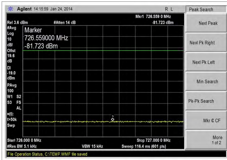
DL_728-746MHz_Low CH_GSM_-20dbm
