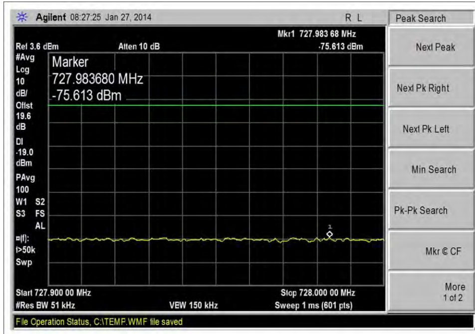
DL_728-746MHz_Low CH_CDMA_-20dbm
