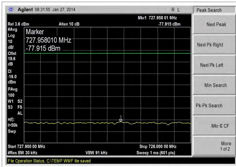
DL_728-746MHz_Low CH_CDMA_-20dbm
