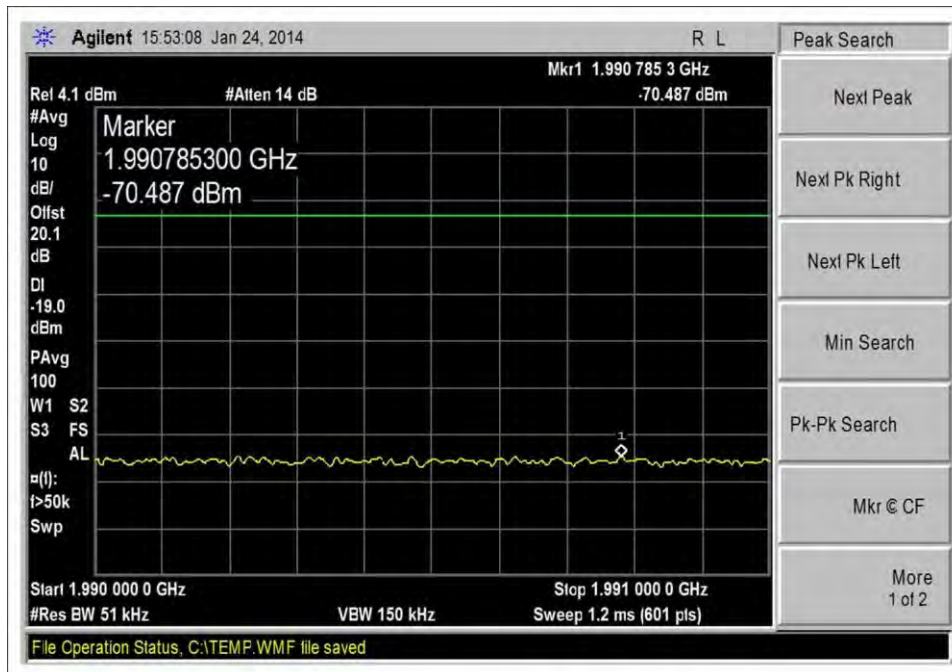
DL_1930-1990MHz_Hi CH_CDMA_-20dbm
