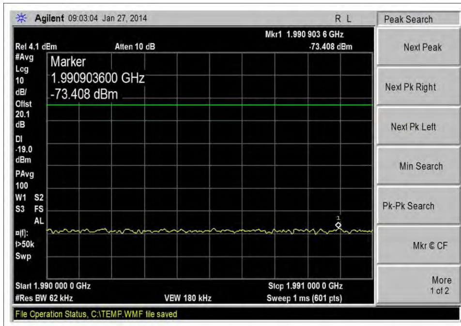
DL_1930-1990MHz_Hi CH_LTE_-20dbm
