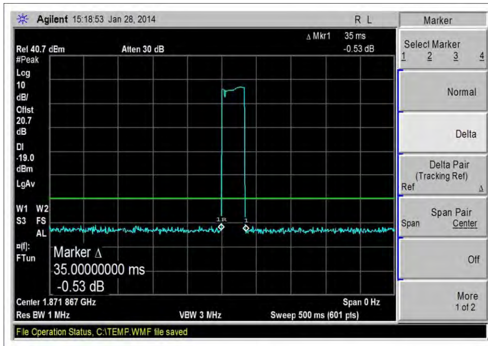
Oscillation Detection_UL_1850-1910MHz
