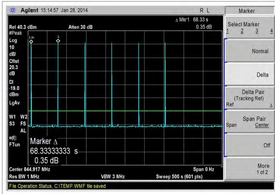
Oscillation Mitigation_UL_824-849MHz
