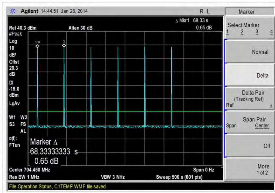
Oscillation Mitigation_UL_698-716MHz
