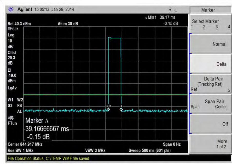
Oscillation Detection_UL_824-849MHz
