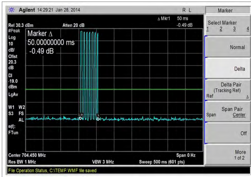
Oscillation Detection_UL_698-716MHz
