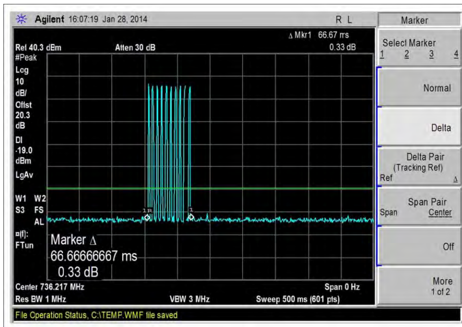
Oscillation Detection_DL_728-746MHz
