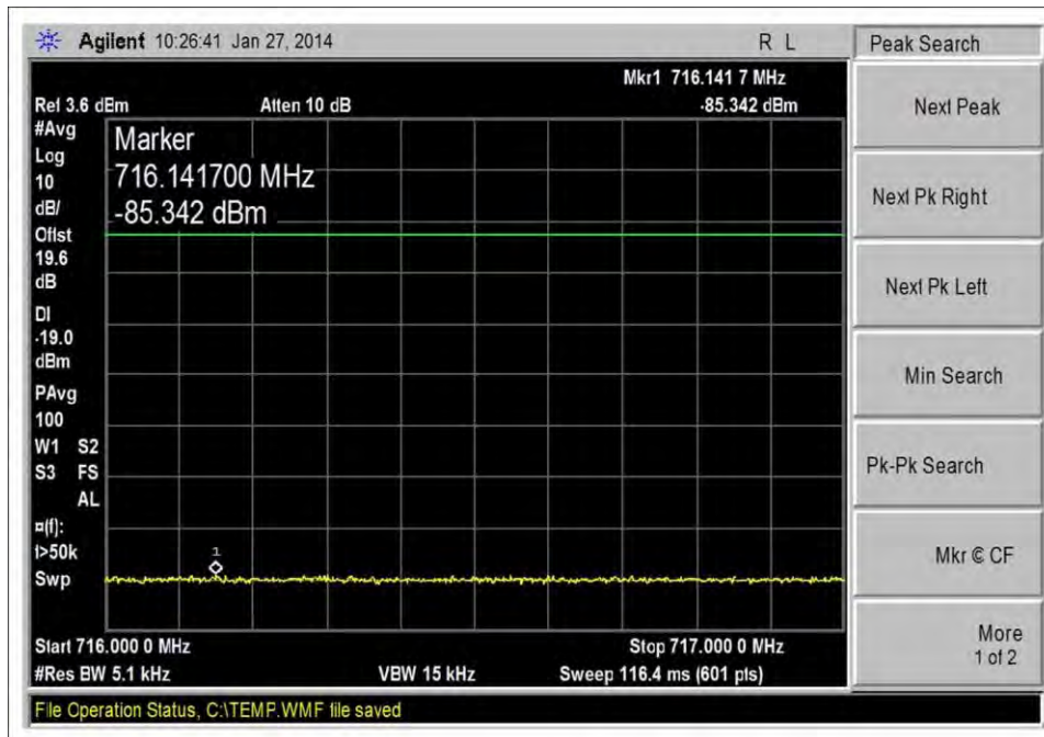
UL_698-716_Hi CH_GSM_10dbm
