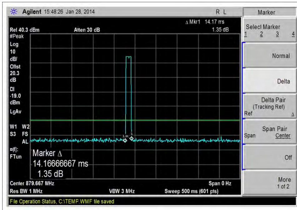
Oscillation Detection_DL_869-894MHz
