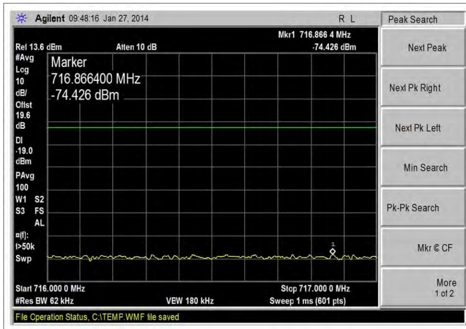
UL_698-716MHz_Hi CH_LTE_10dbm
