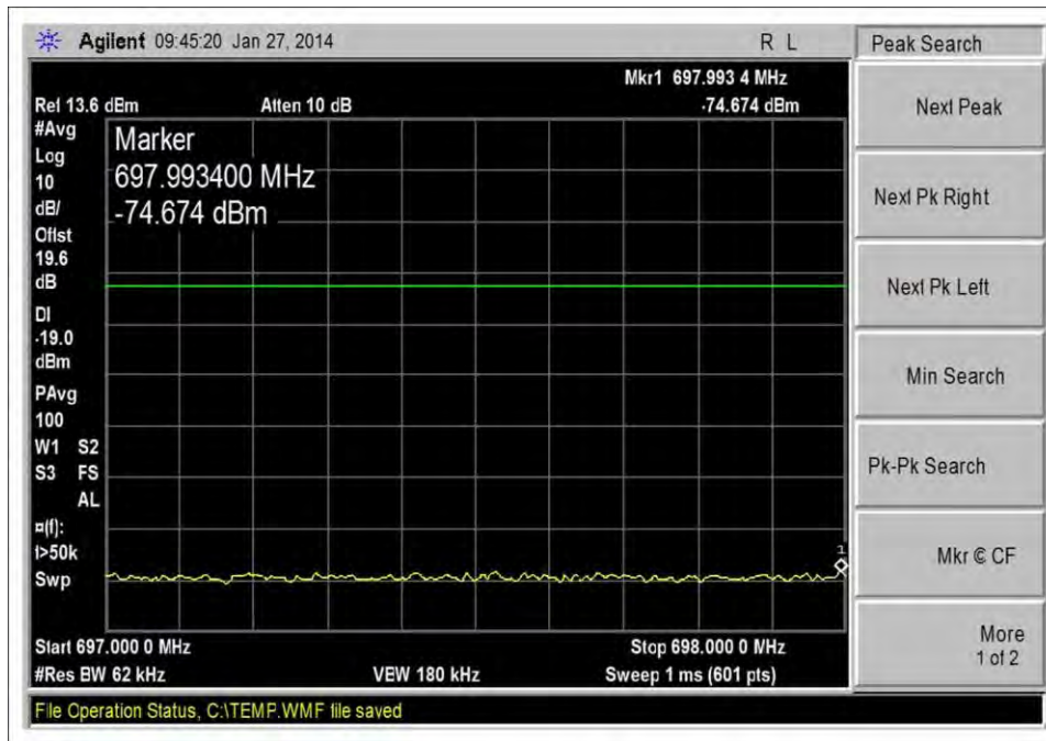
UL_698-716MHz_Low CH_LTE_10dbm
