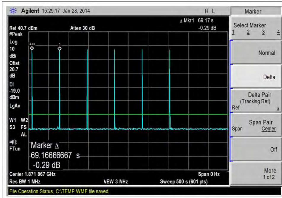
Oscillation Mitigation_UL_1850-1910MHz
