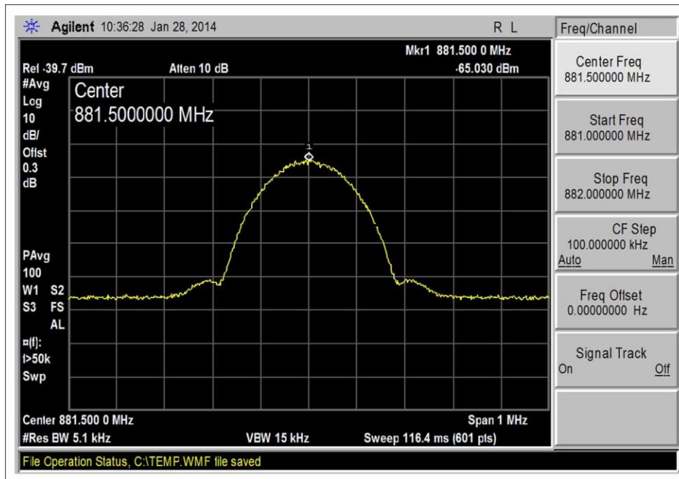
GSM_DL 869-894_Input
