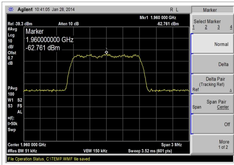
CDMA_DL 1930-1990_Input
