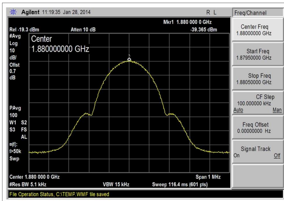
GSM_UL 1850-1910_Input
