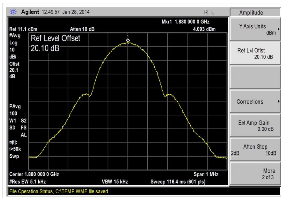
GSM_UL 1850-1910_Output
