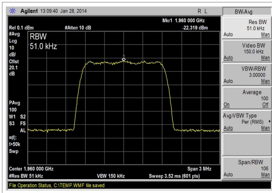
CDMA_DL 1930-1990_Output
