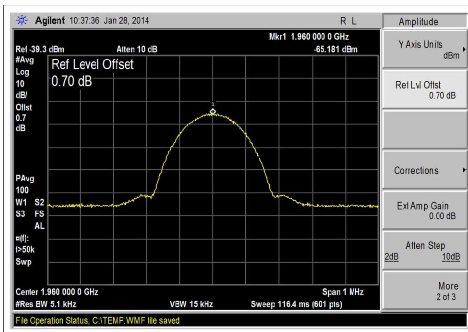
GSM_DL 1930-1990_Input
