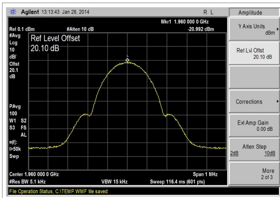
GSM_DL 1930-1990_Output
