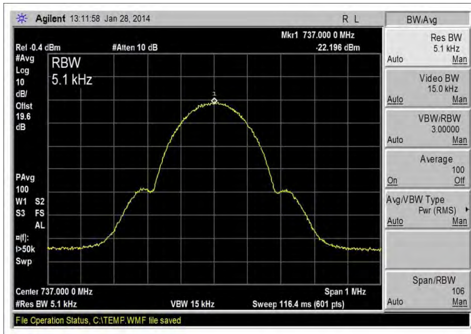
GSM_DL 728-746_Output
