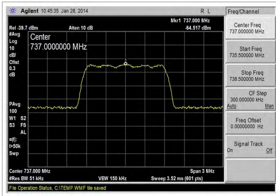
CDMA_DL 728-746_Input
