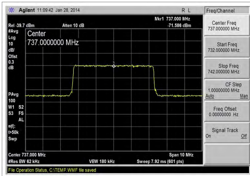
LTE_DL 728-746_Input
