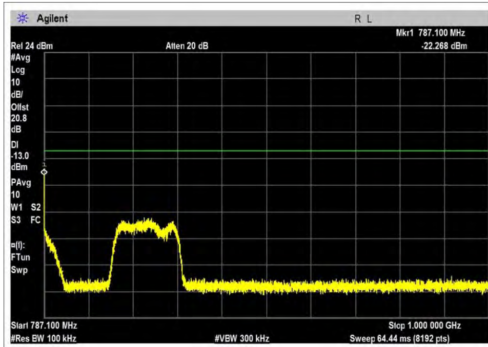
UL-776-787R-GSM-H
