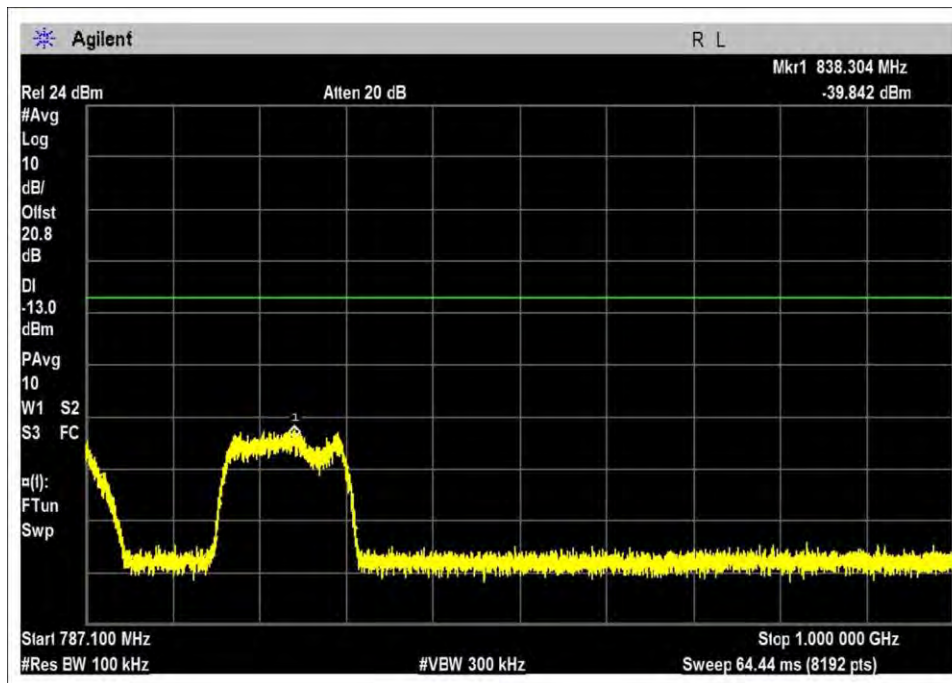
UL-776-787R-GSM-L
