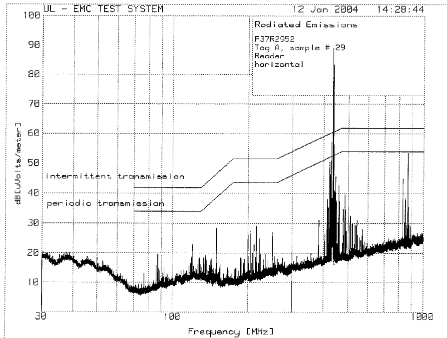
Radiated Emissions, 30 – 1000 MHz horizontal peak prescan
