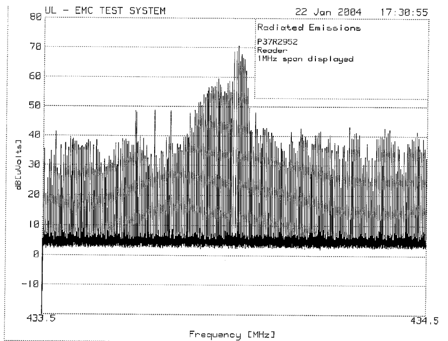
Tag Reader, 1MHz span shown
