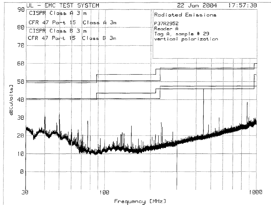
30-1000MHz, vertical prescan
