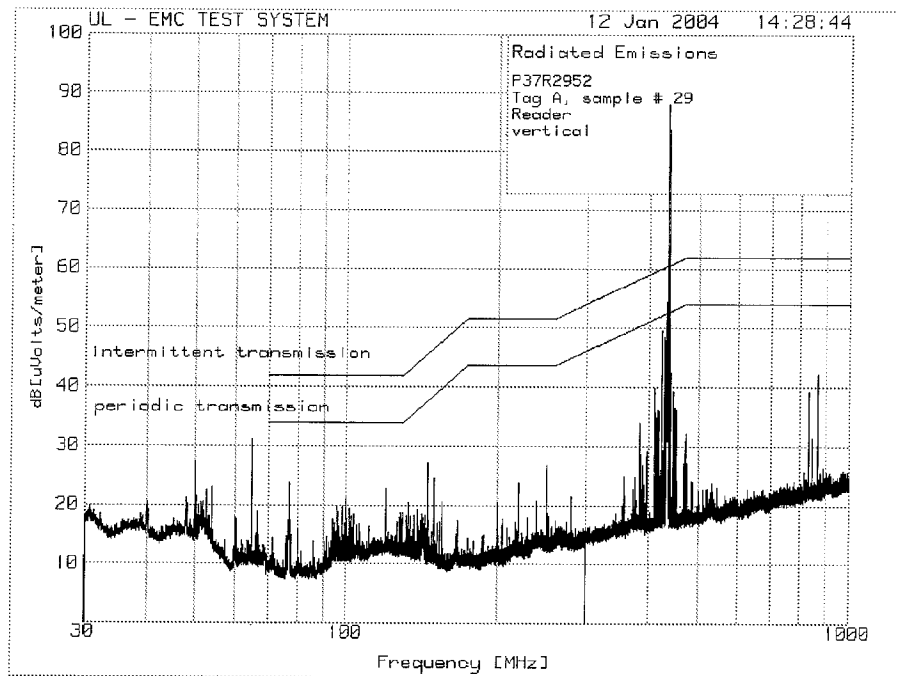
30 – 1000 MHz vertical peak prescan, Tag Reader & Sensor Tag A
