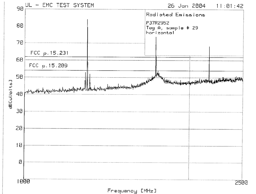
1 – 2.5 GHz horizontal peak prescan. Sensor Tag A
