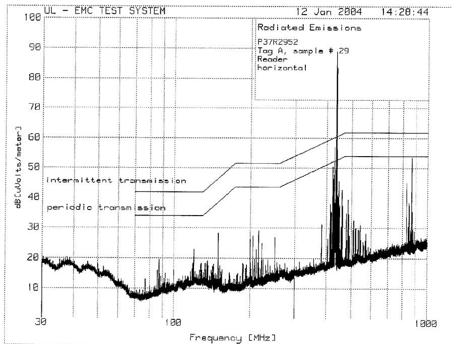
30 – 1000 MHz horizontal peak prescan, Tag Reader & Sensor Tag A
