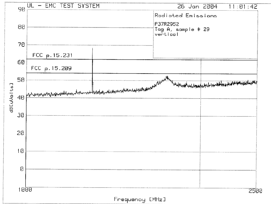
1 – 2.5 GHz vertical peak prescan. Sensor Tag A
