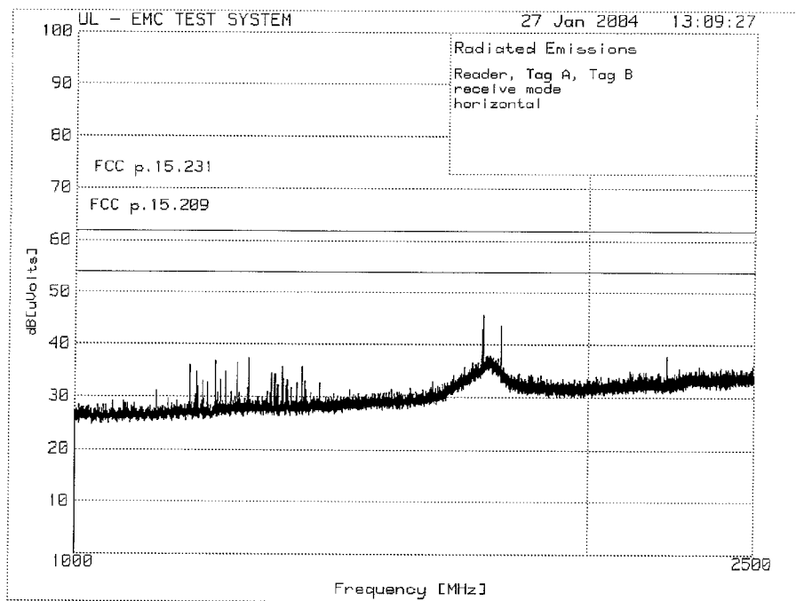
Radiated Emissions 1-2.5GHz, horizontal prescan
