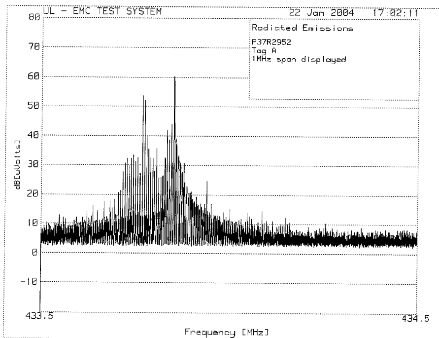
Sensor Tag A, 1MHz span shown
