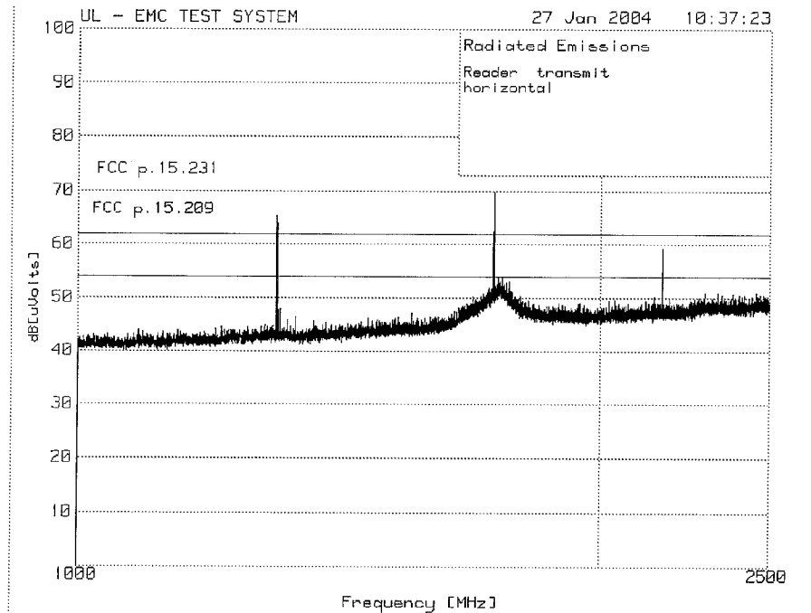
1 – 2.5 GHz horizontal peak prescan. Tag Reader
