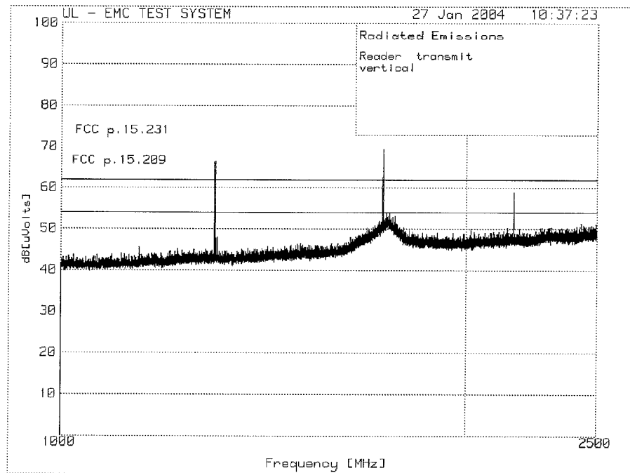
1 – 2.5 GHz vertical peak prescan. Tag Reader
