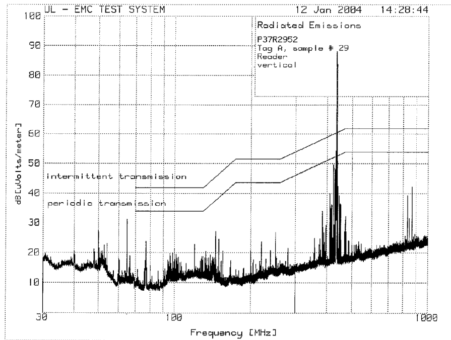
Radiated Emissions, 30 – 1000 MHz vertical peak prescan
