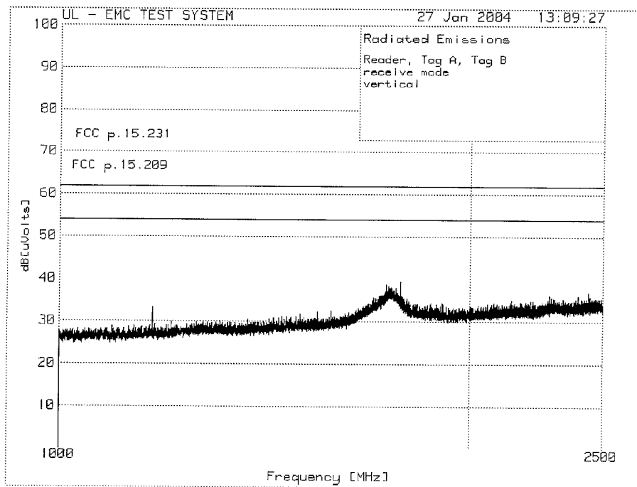
1-2.5GHz, vertical prescan
