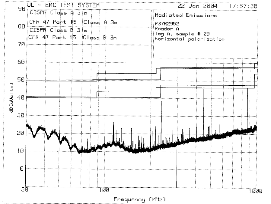
30-1000MHz, horizontal prescan
