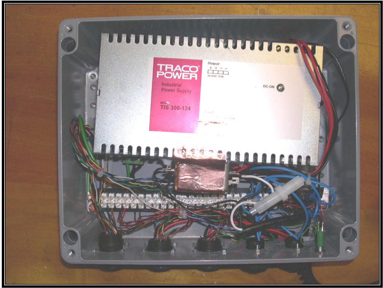
PHOTOGRAPH 39: POWER SUPPLY-GENERAL INSIDE VIEW
