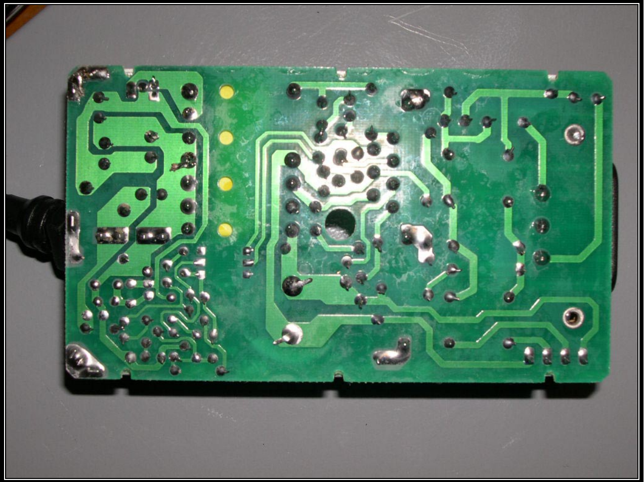
PHOTOGRAPH 43: POWER SUPPLY–BOTTOM VIEW AC/DC CONVERTER
