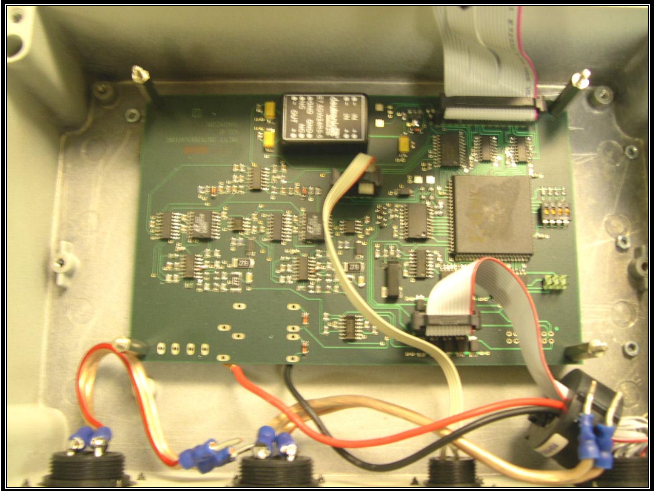
PHOTOGRAPH 36: ADU 2-SECOND BOARD INSIDE UNIT
