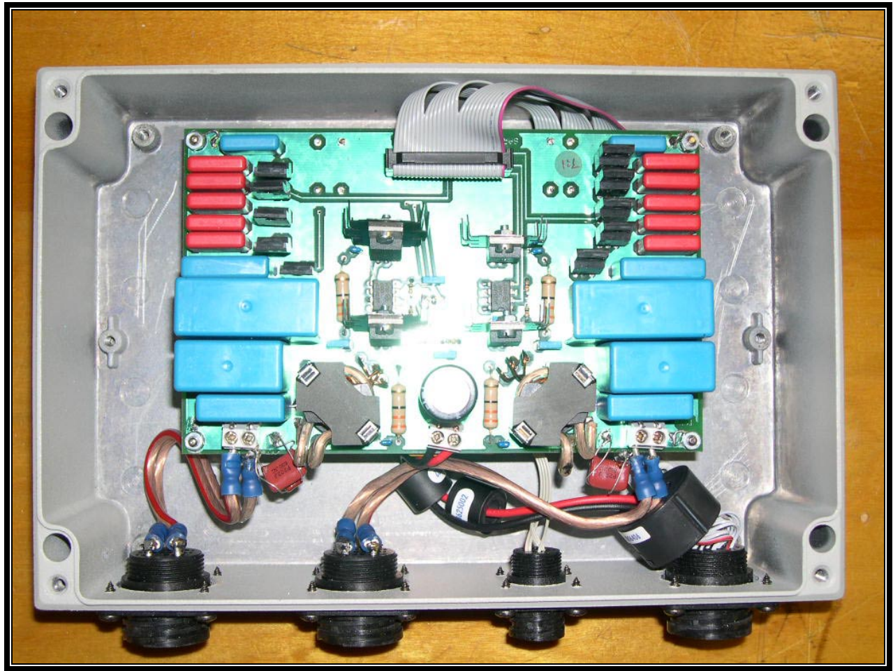
PHOTOGRAPH 27: ADU 1—GENERAL INSIDE VIEW
