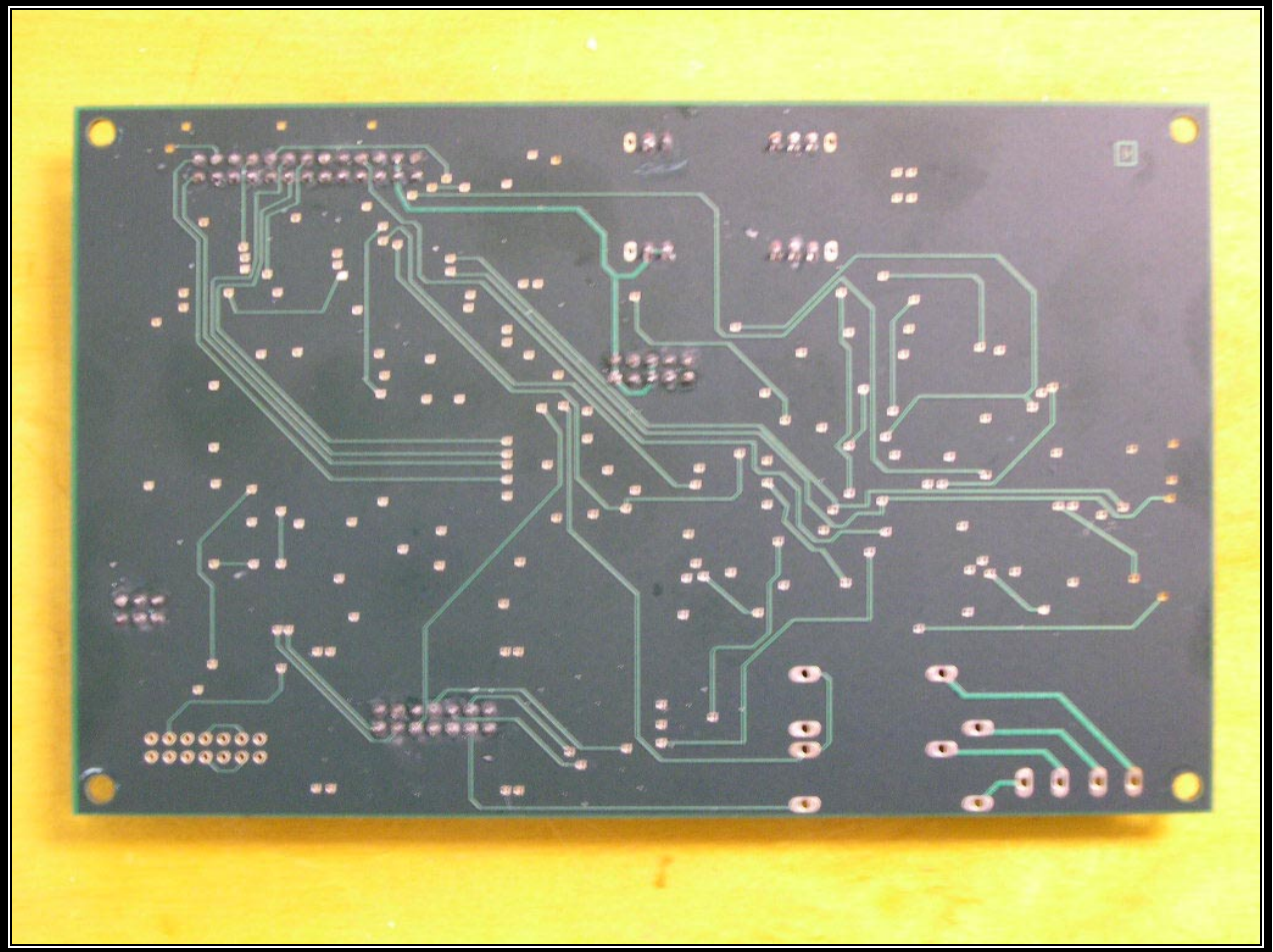
PHOTOGRAPH 32: ADU 1-SECOND BOARD BOTTOM VIEW
