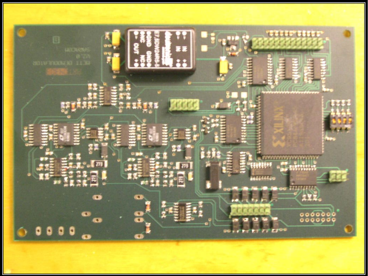
PHOTOGRAPH 31: ADU 1-SECOND BOARD TOP VIEW
