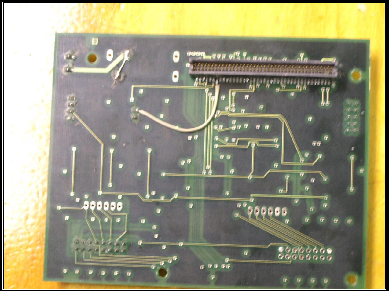
PHOTOGRAPH 47: DPU-BOTTOM VIEW
