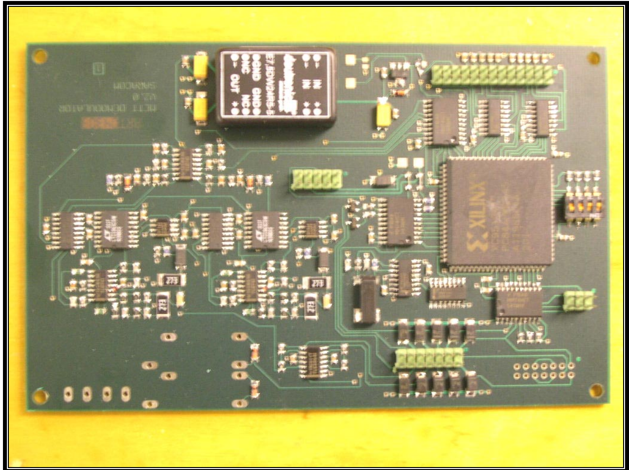
PHOTOGRAPH 37: ADU 2-SECOND BOARD TOP VIEW
