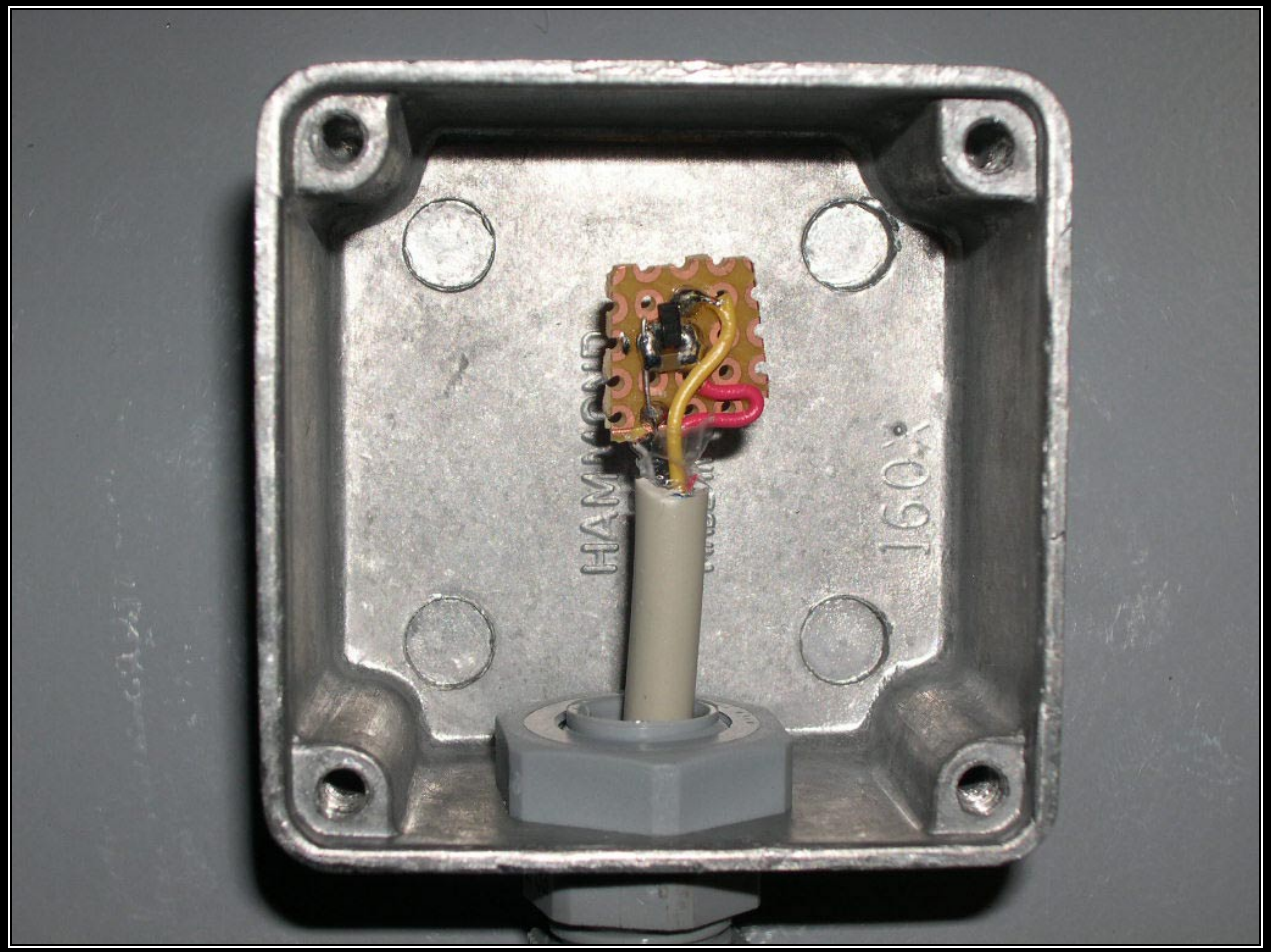
PHOTOGRAPH 44: SENSOR-TOP VIEW
