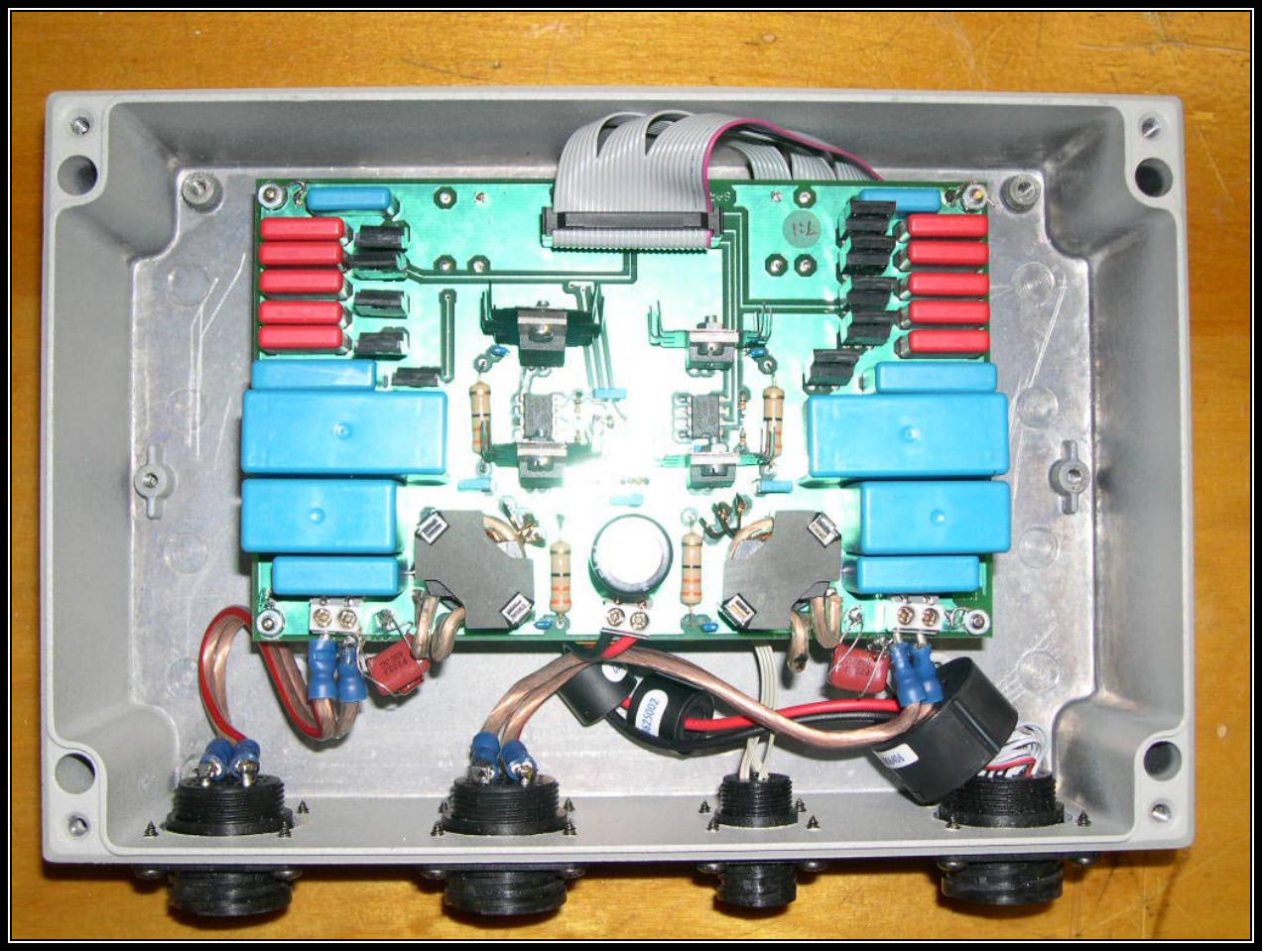
PHOTOGRAPH 33: ADU 2—GENERAL INSIDE VIEW
