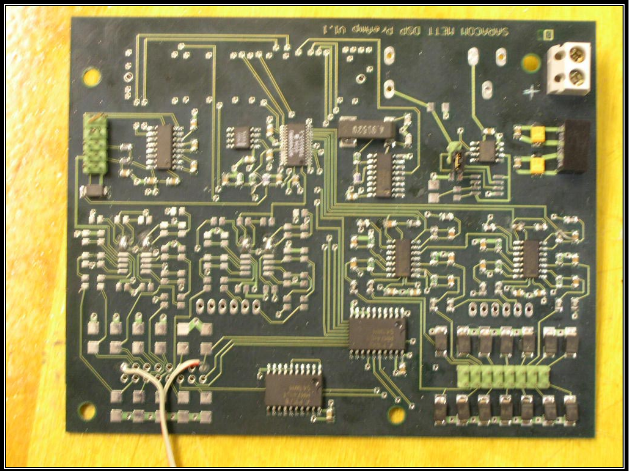
PHOTOGRAPH 46: DPU-TOP VIEW
