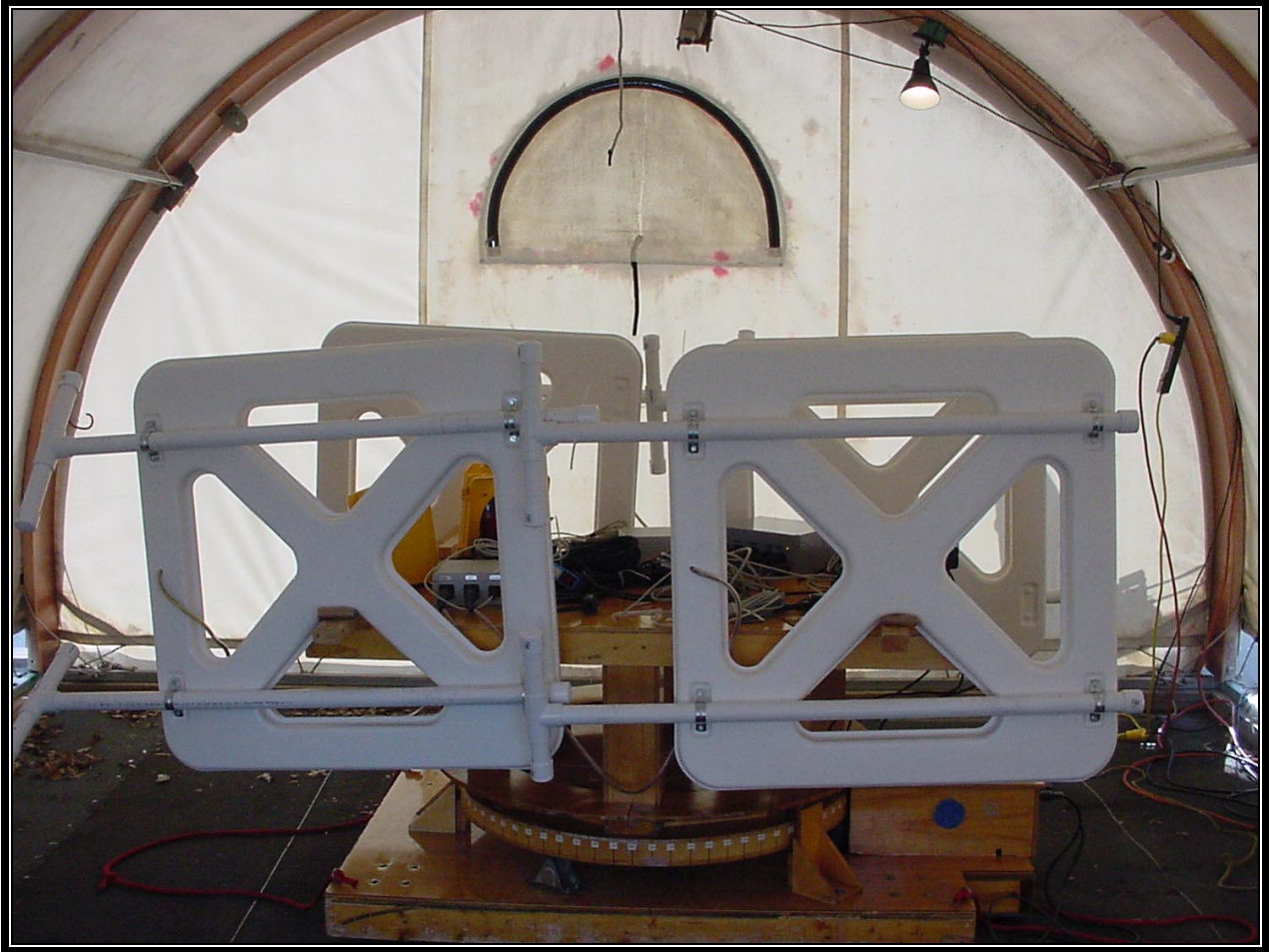
PHOTOGRAPH 4: RADIATED EMISSIONS REAR VIEW
