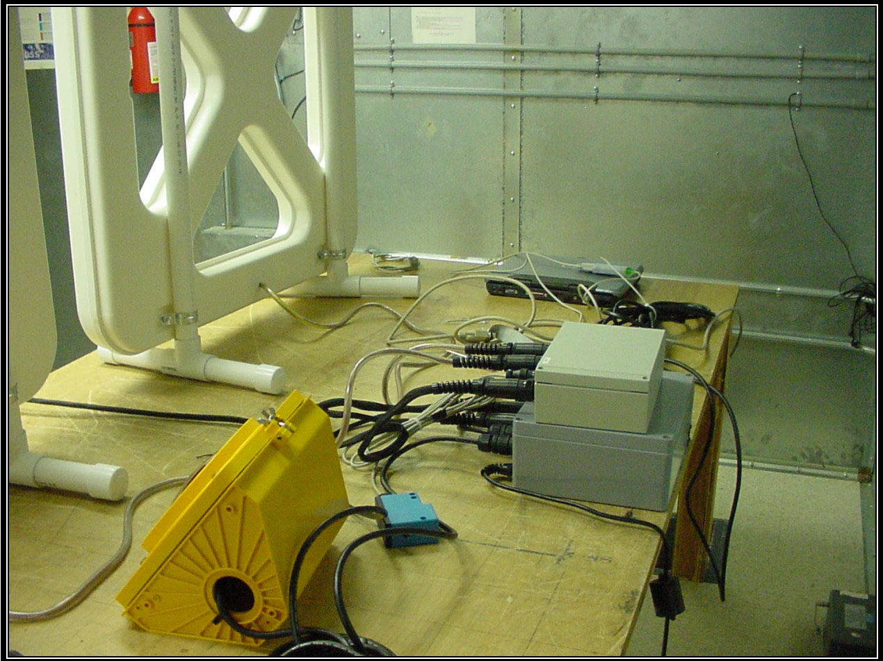
PHOTOGRAPH 6: CONDUCTED EMISSIONS REAR VIEW
