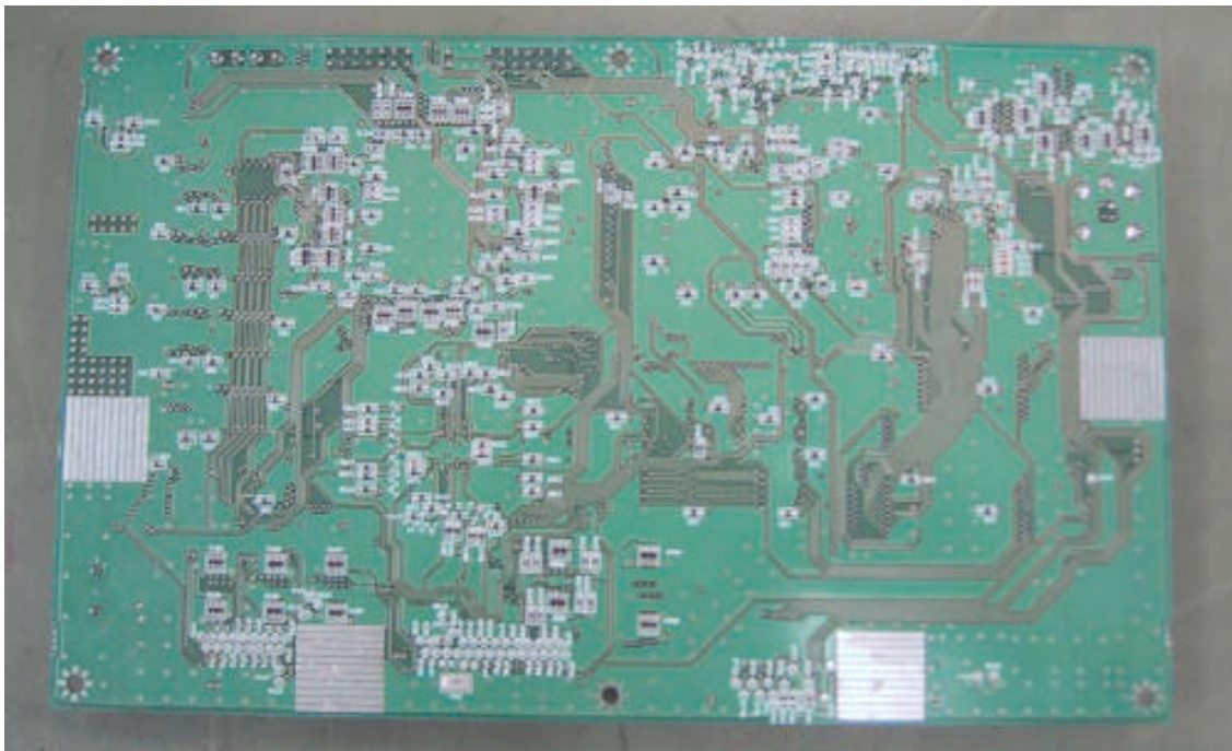
Photograph 21 – Bottom View of the Main PCB
