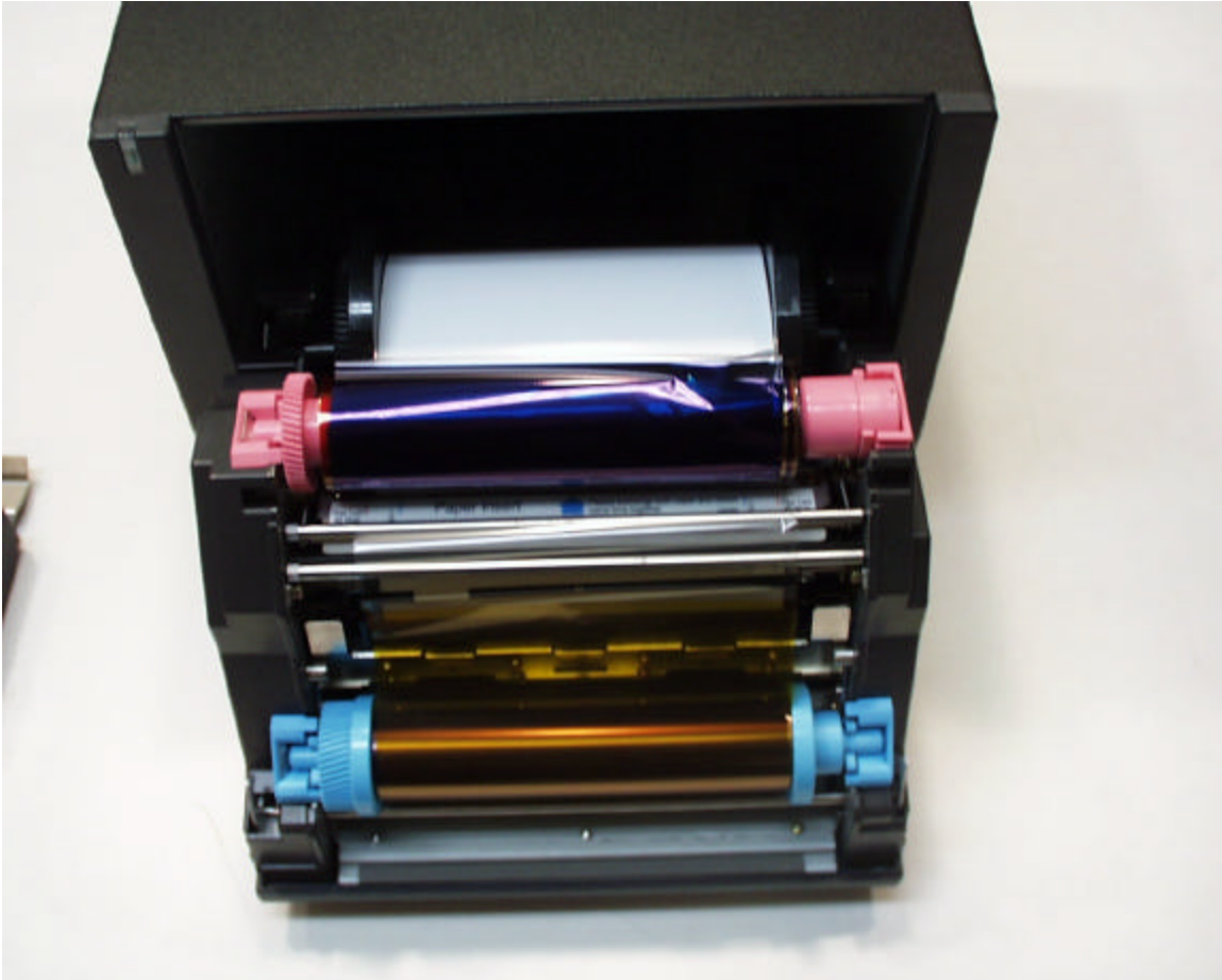
Photograph 16 – View of the CV01-H01 with Front Cover Open Showing Placement of the RFID Tag In the Printer
