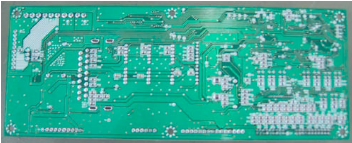
Photograph 19 – Bottom View of the Driver PCB
