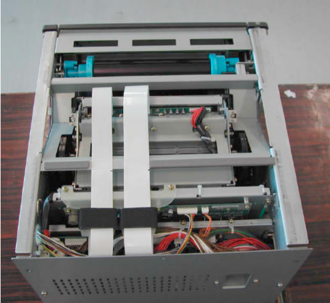
Photograph 1 – Internal Top View of the CV01-H01
