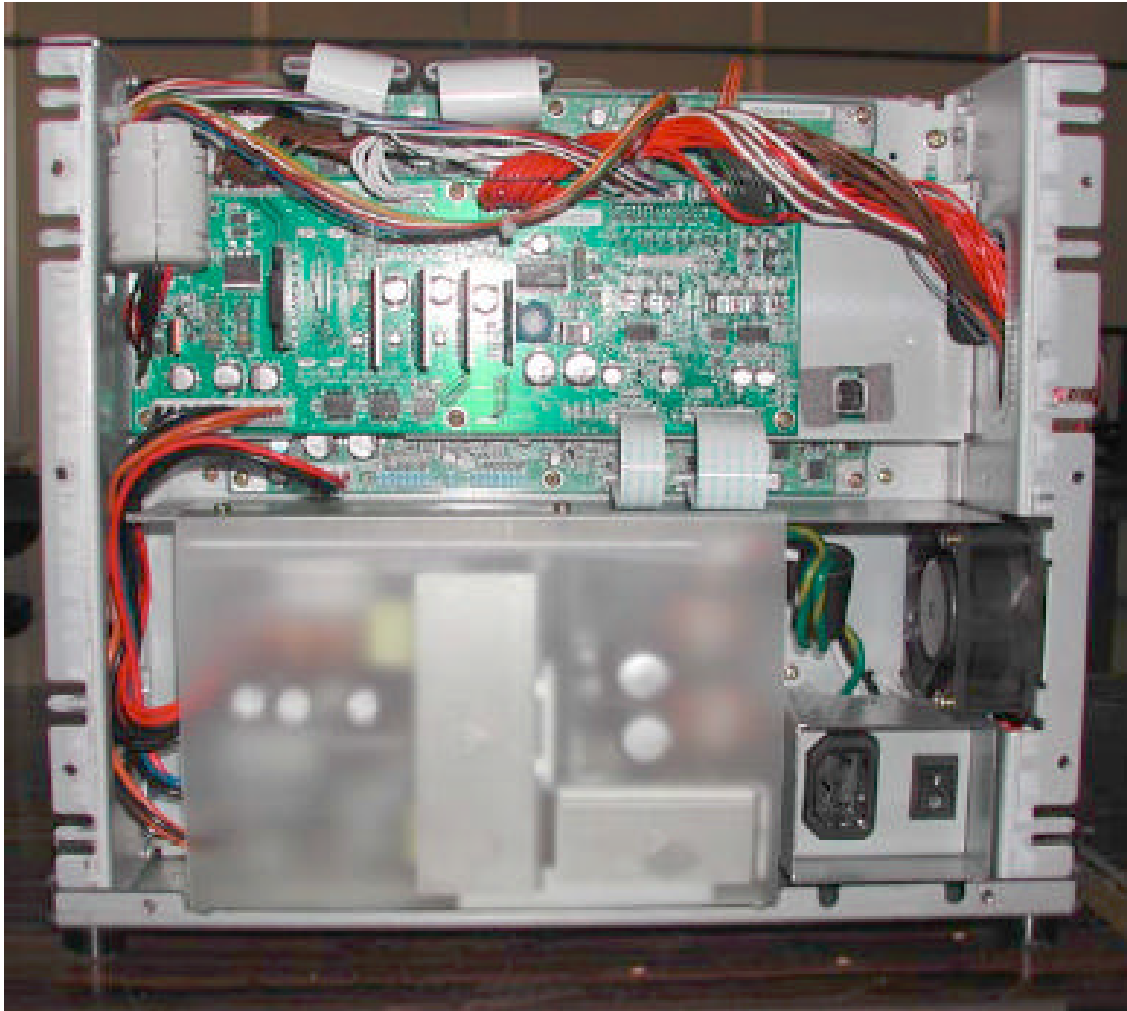
Photograph 5 – Internal Back View of the CV01-H01
