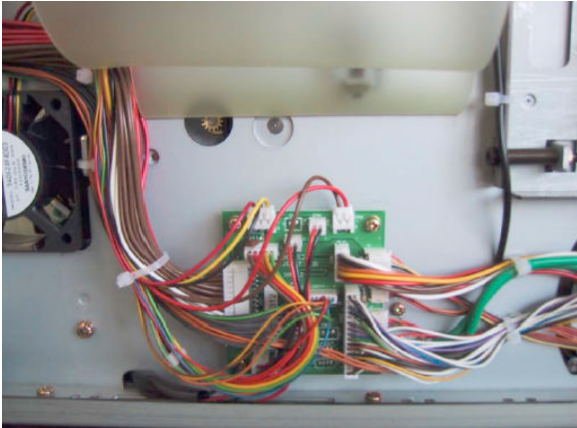
Photograph 4 – Internal Left Side View of the CV01-H01 with Cover Removed
