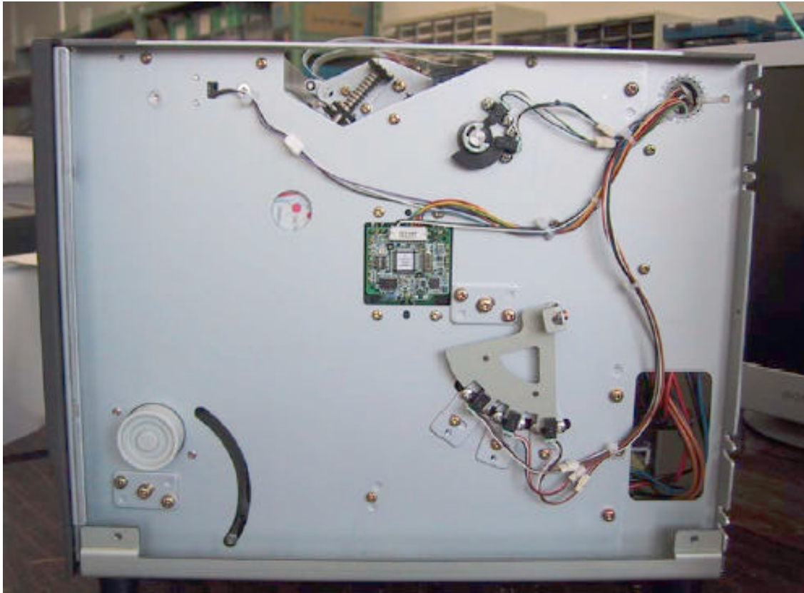
Photograph 2 – Internal Right Side View of the CV01-H01
