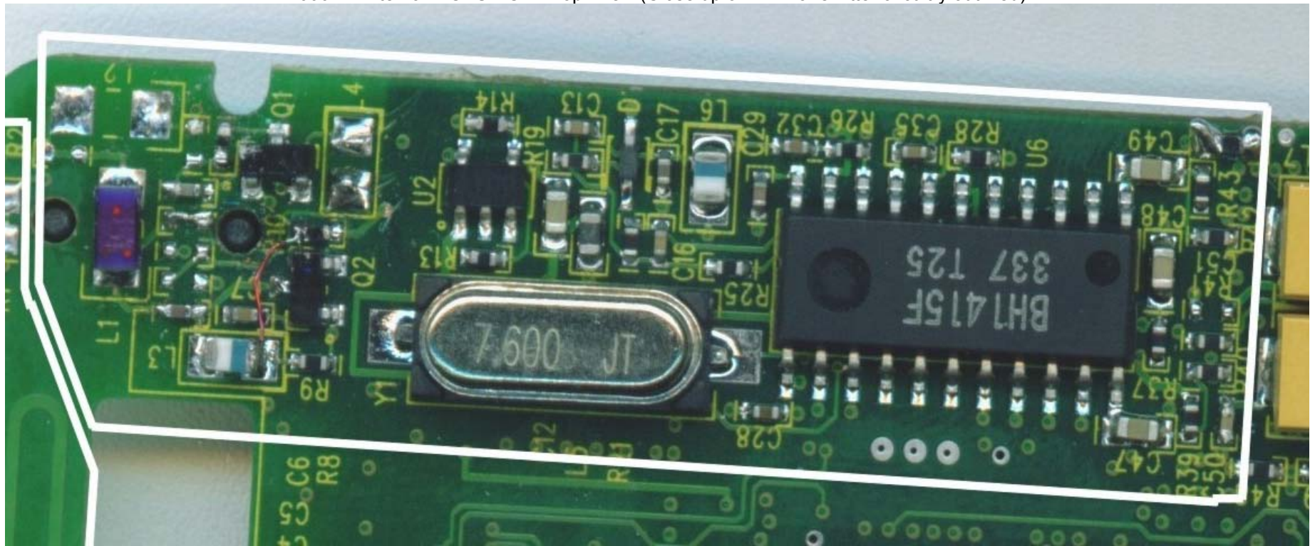
1000FM Internal - CPU PCB - Top View (Close up of FM Transmitter circuitry outlined)
