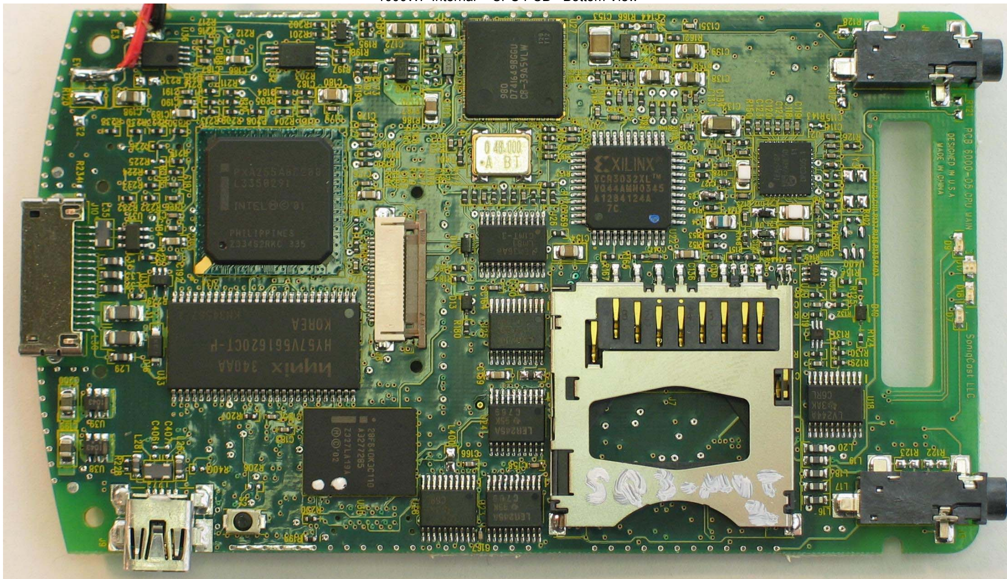
1000WF Internal - CPU PCB - Bottom View
