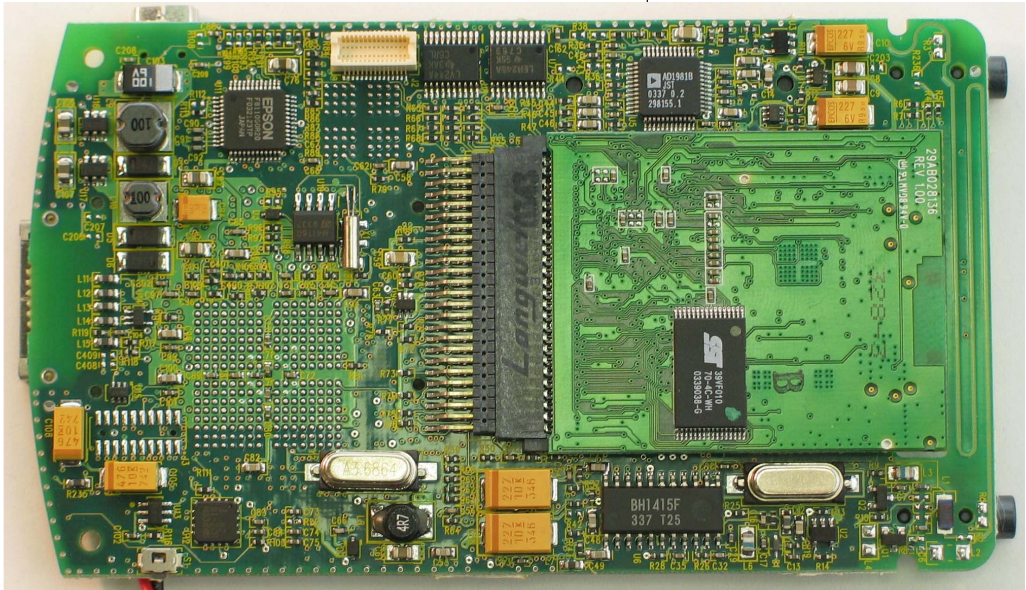
1000WF Internal - CPU PCB with WIFI Board - Top View
