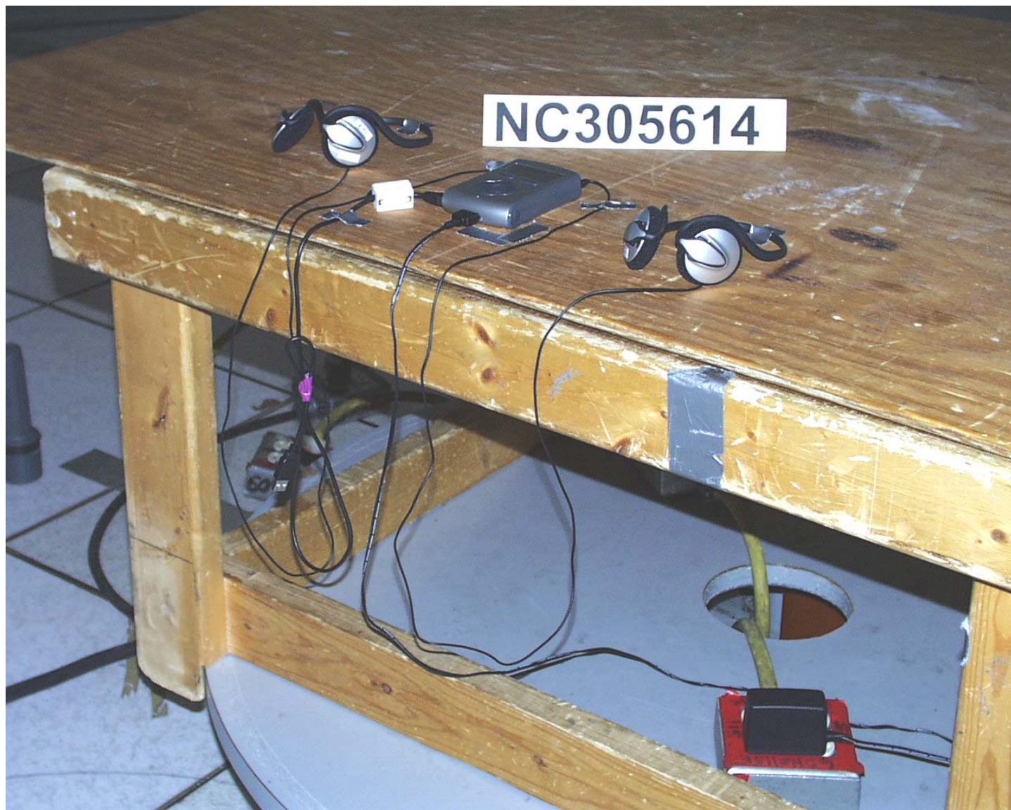
Test-setup photo(s): Radiated emission 30 MHz - 25000 MHz
