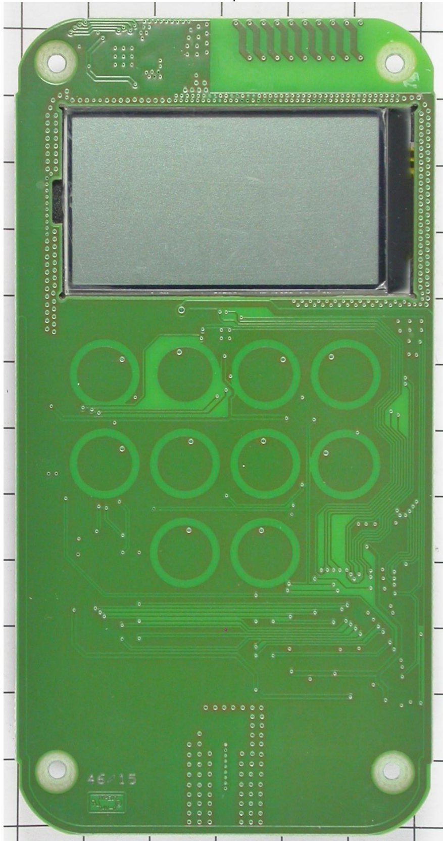
PCB – top view
