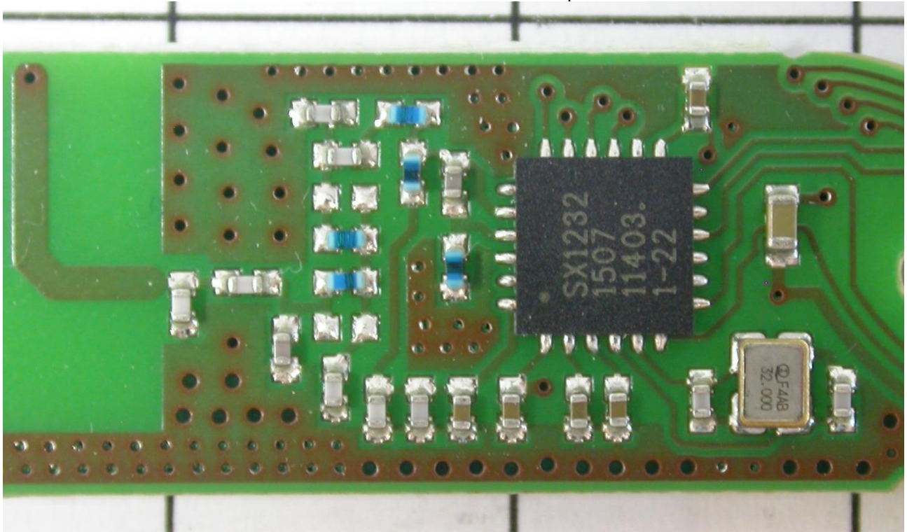
Detailed bottom view of the RF part
