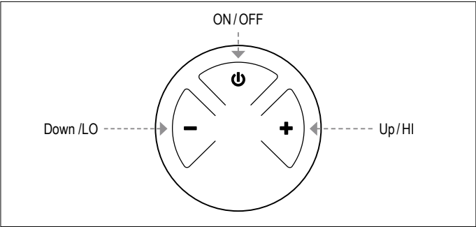
Figure 23: 3-button layout
