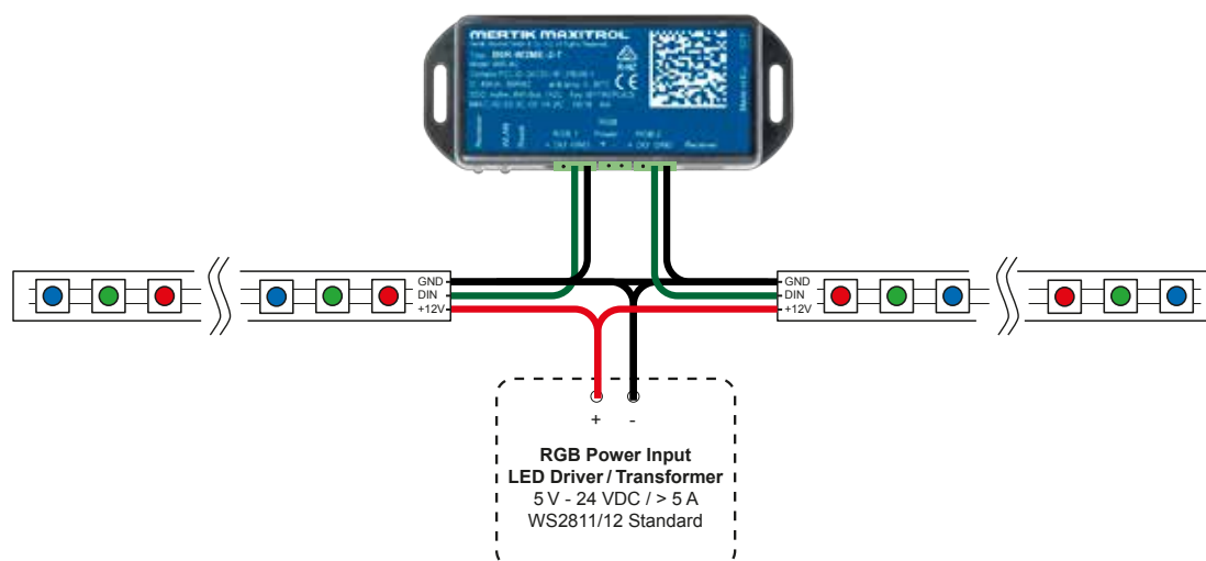
Figure 26: LED setup 2 (Indirect connection)
