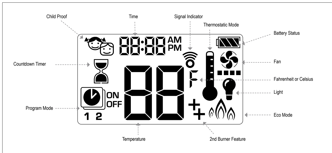
Figure 22: 10-button Display
