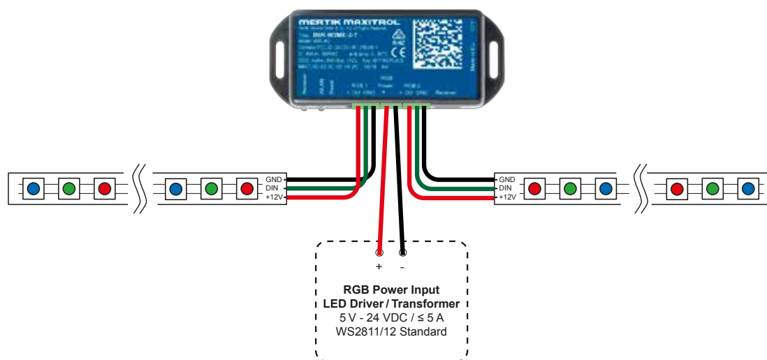
Figure 25: LED setup 1 (Direct connection)
