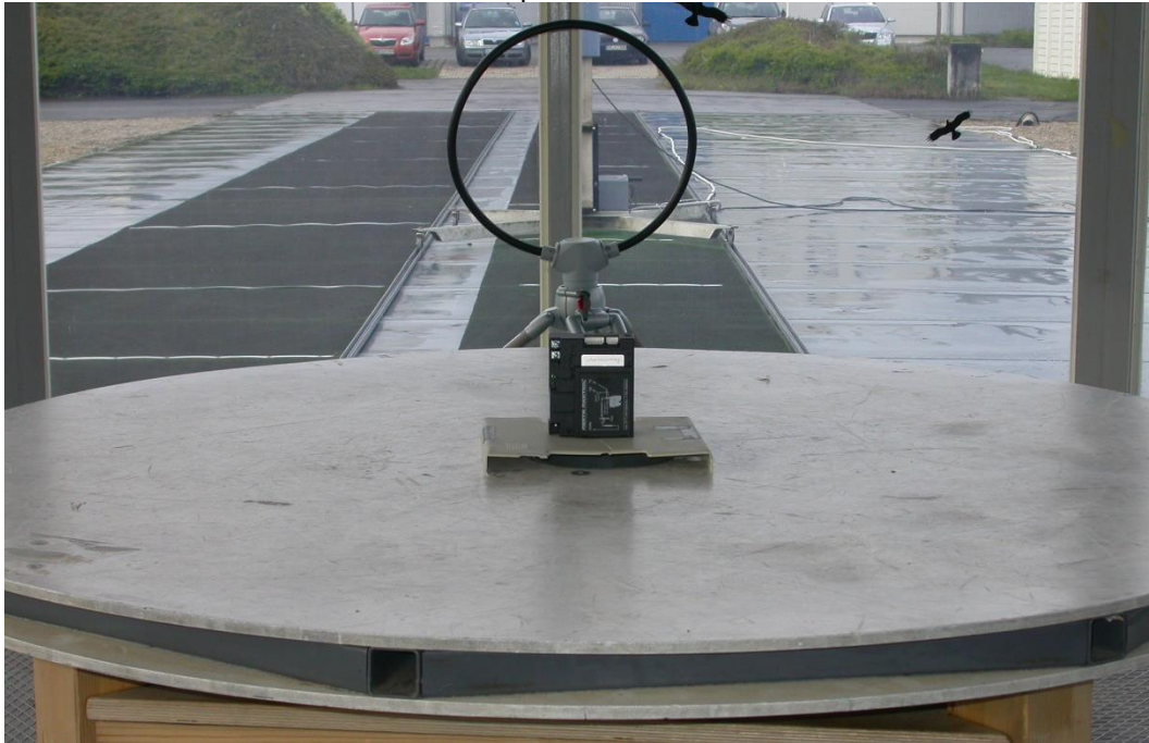
Test setup 9 kHz – 30 MHz:
