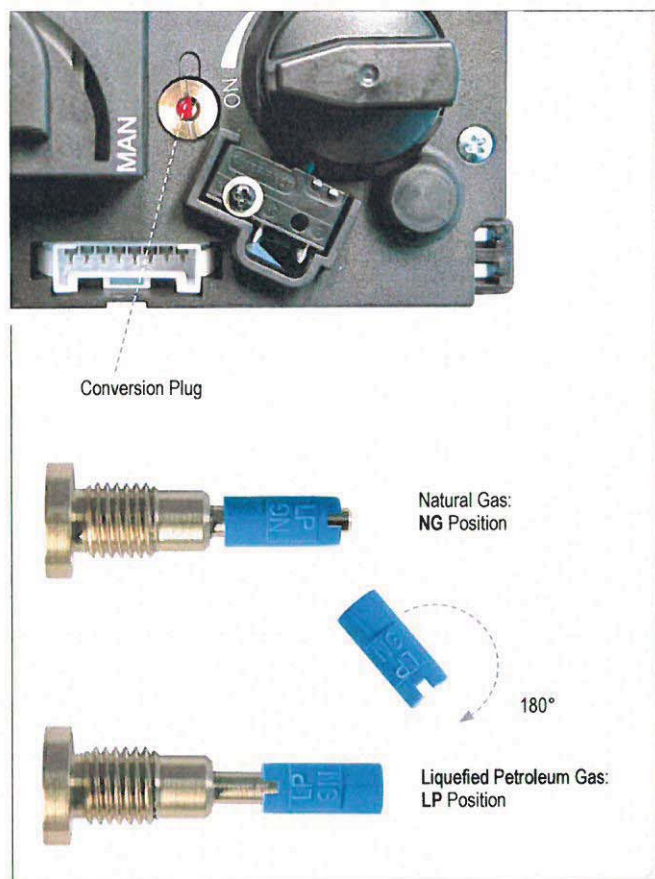
Figure 24: Conversion from one gas to another
