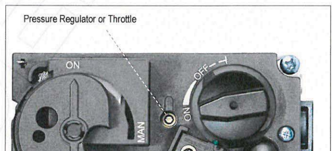
Figure 23: Combination Control GV60, Cover
