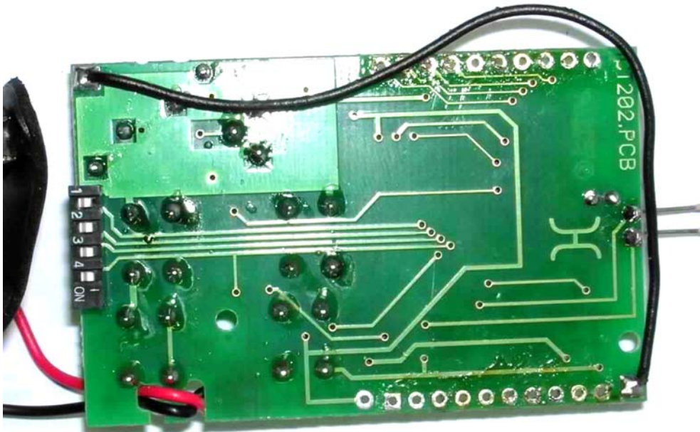
Internal Photo Rear view PCB
