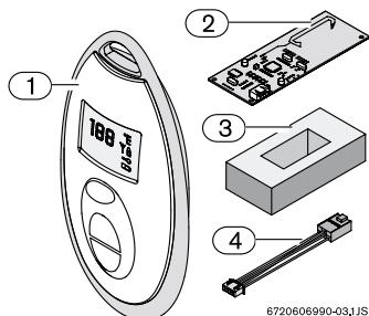
Fig. 1 Parts
