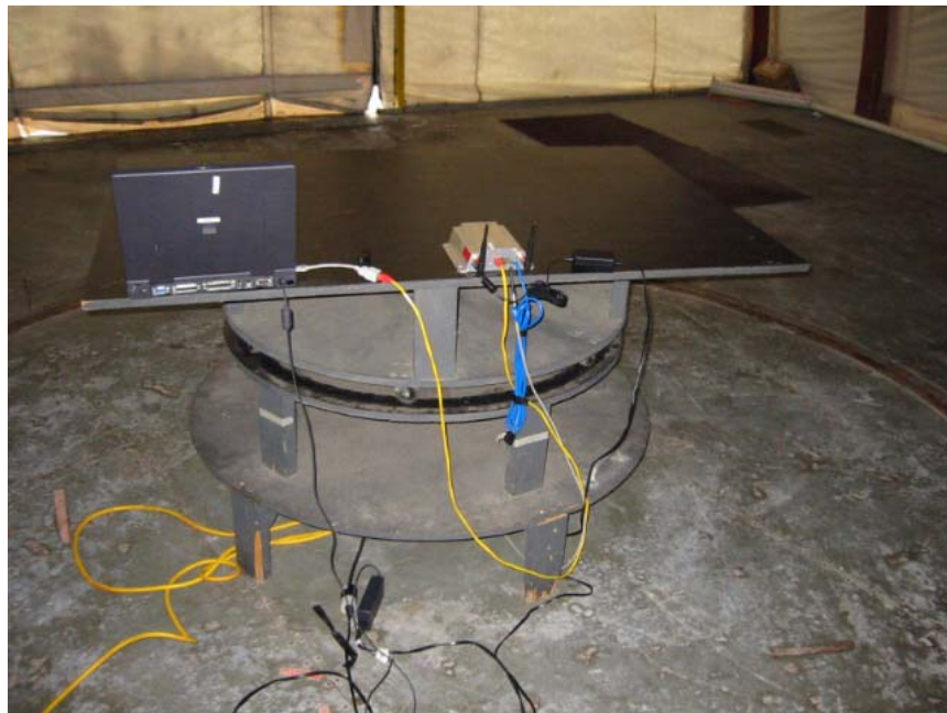
Radiated Spurious Test Setup, Back View
