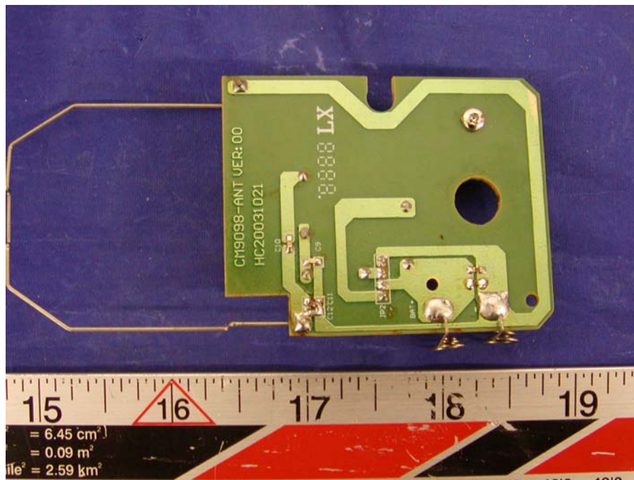
EUT - Component View (Board II)
