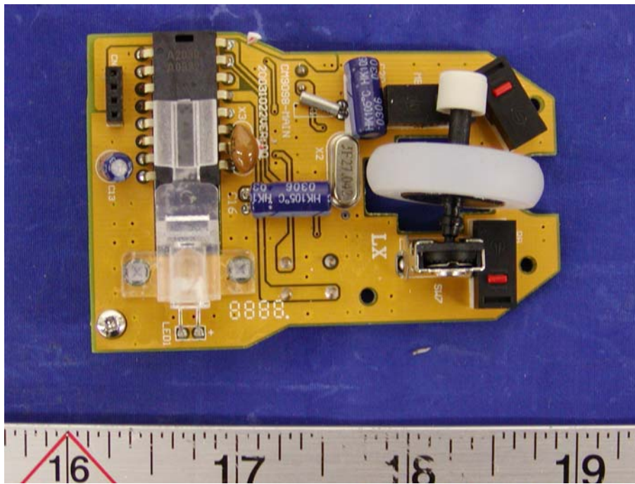
EUT - Component View (Board I)
