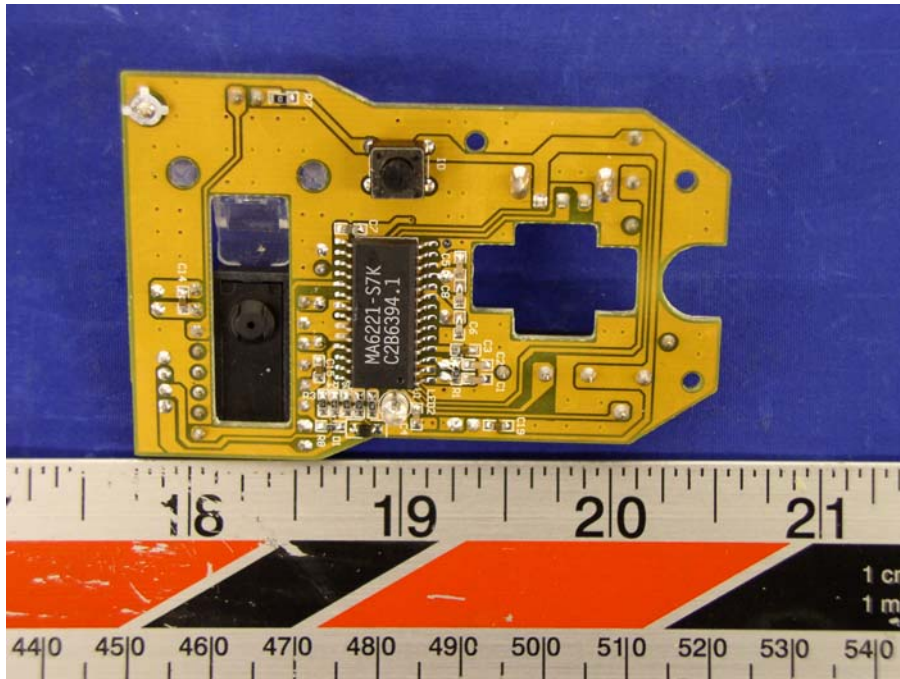
EUT - Solder View (Board I)
