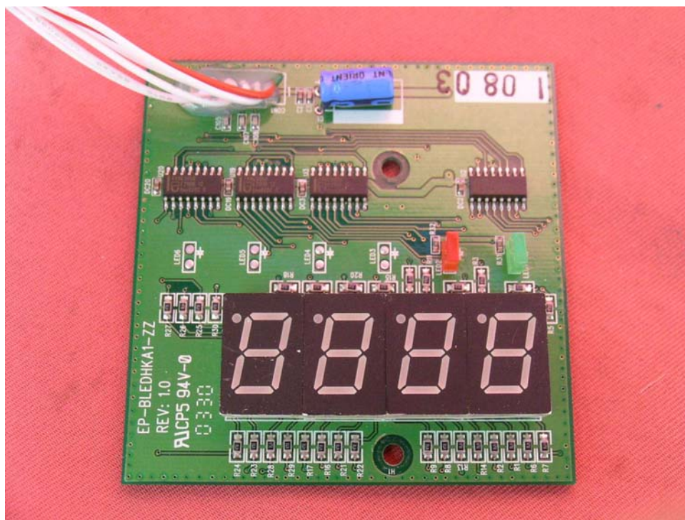
Base display front side
