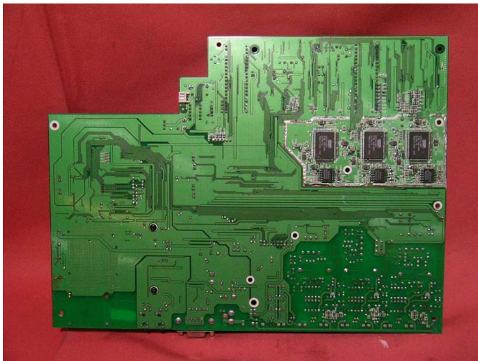
Base Main PCB solder side (View 2)
