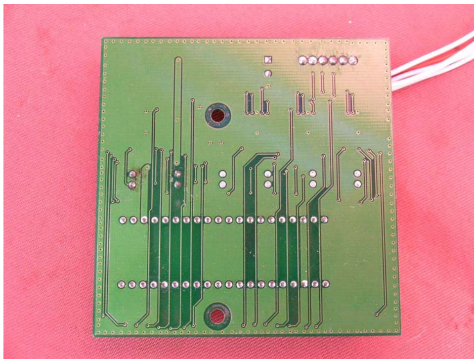
Base display rear side
