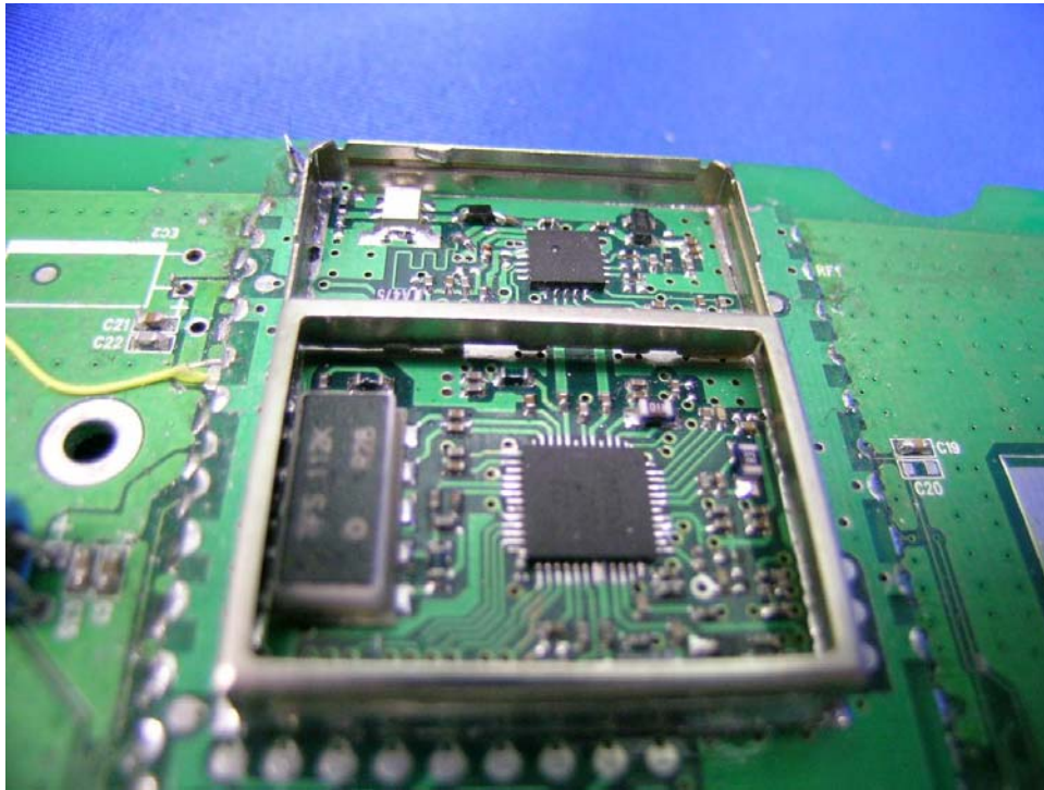
Desktop Oscillator PCB comp side (View 3)
