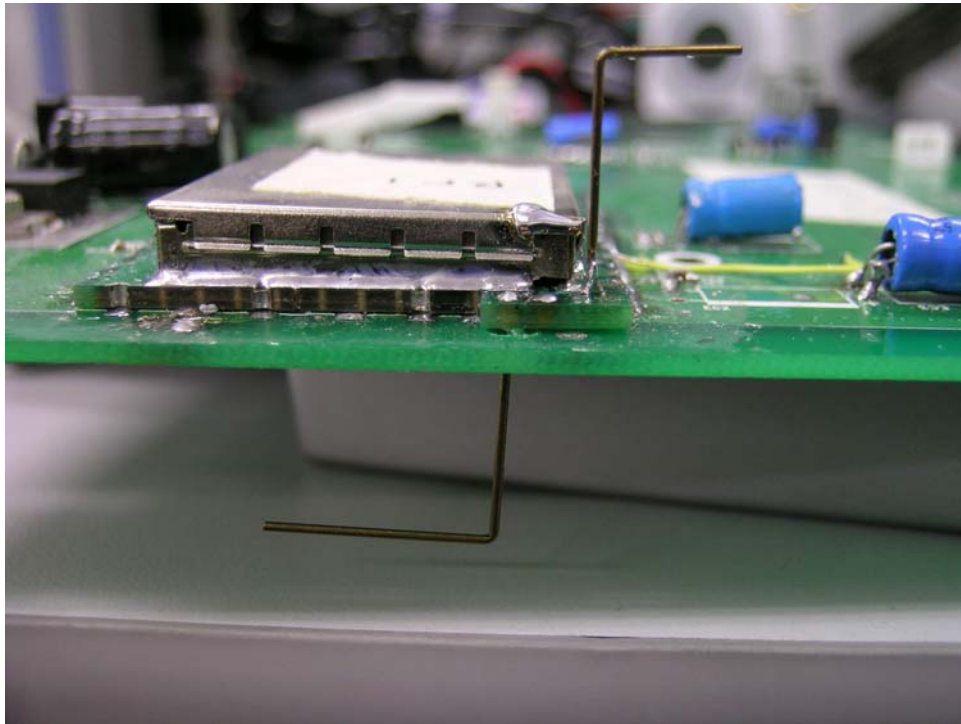
Desktop Main PCB comp side (View 2)
