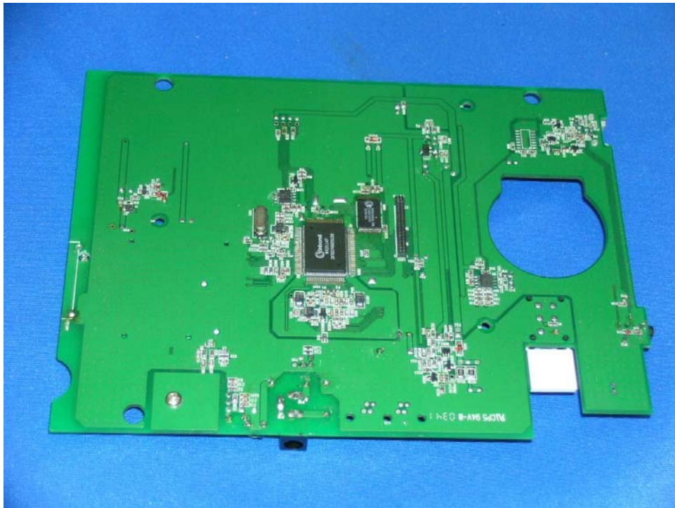
Desktop Main PCB solder side
