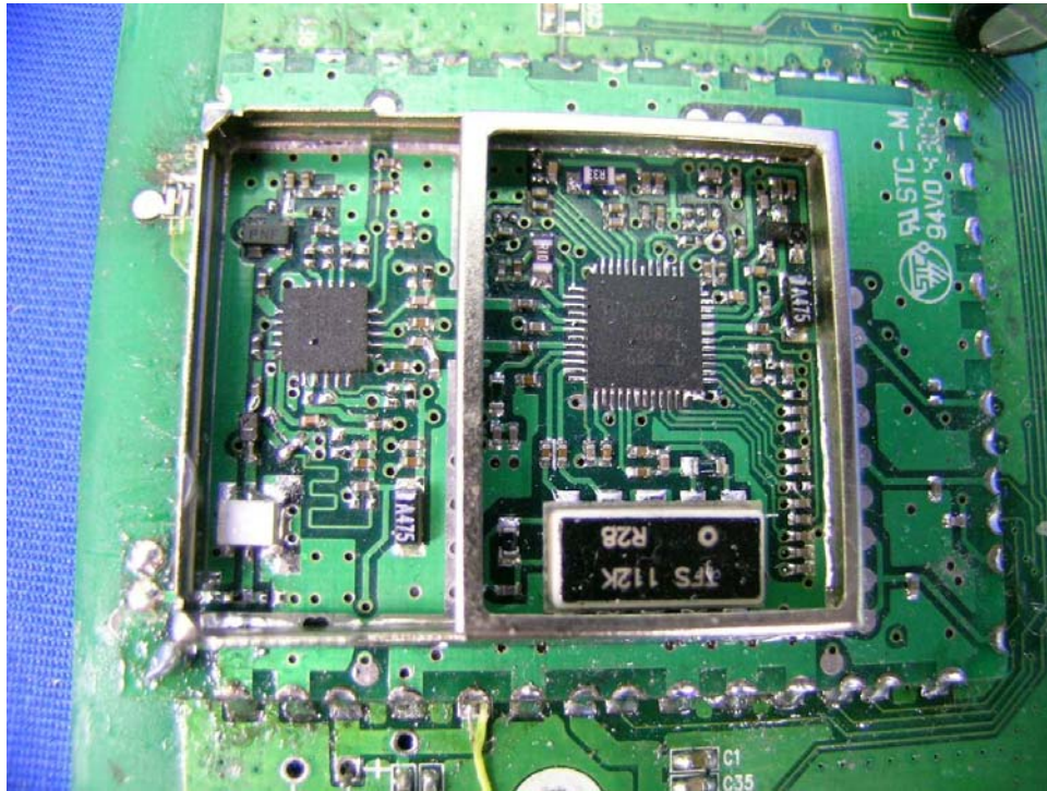
Desktop Oscillator PCB comp side (View 1)
