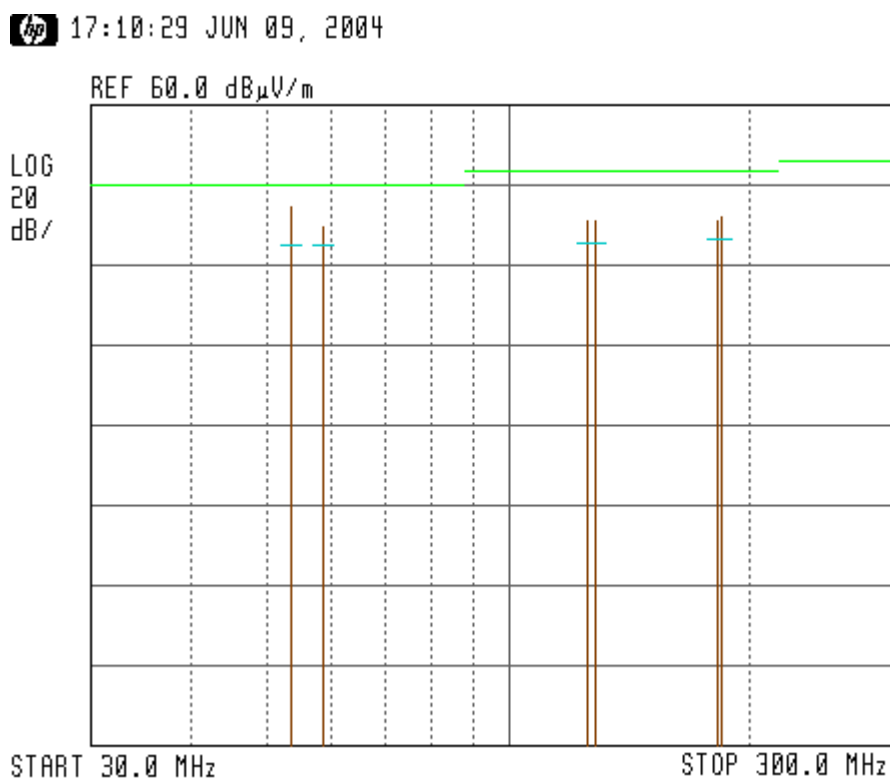
Figure 3. Radiated Emission. Antenna Polarization: HORIZONTAL Detectors: Peak, Quasi-peak
