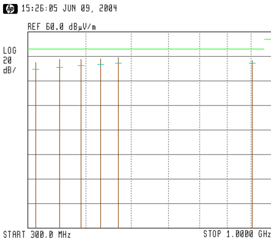
Figure 11. Radiated Emission. Antenna Polarization: VERTICAL. Detectors: Peak, Quasi-peak
