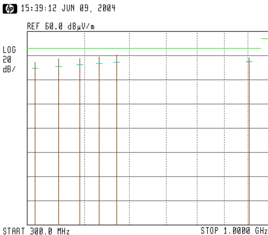
Figure 5. Radiated Emission. Antenna Polarization: HORIZONTAL Detectors: Peak, Quasi-peak
