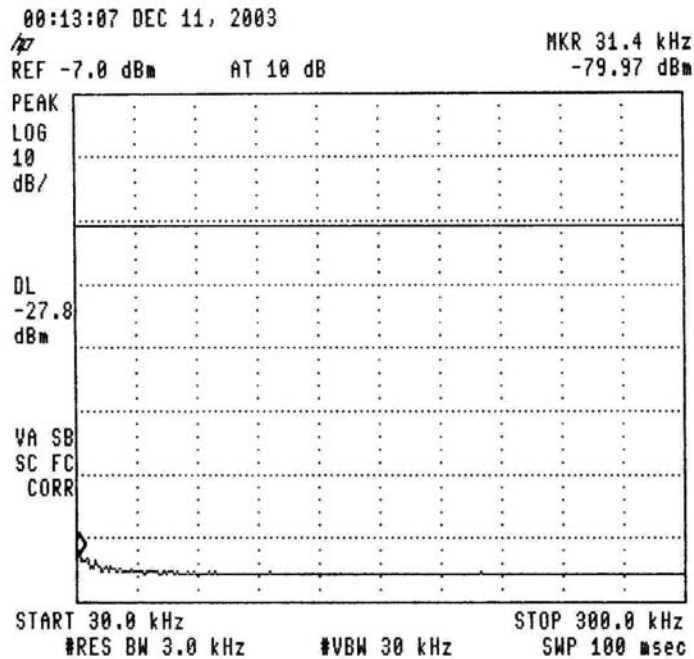
Figure 26.— 913.5 MHz
