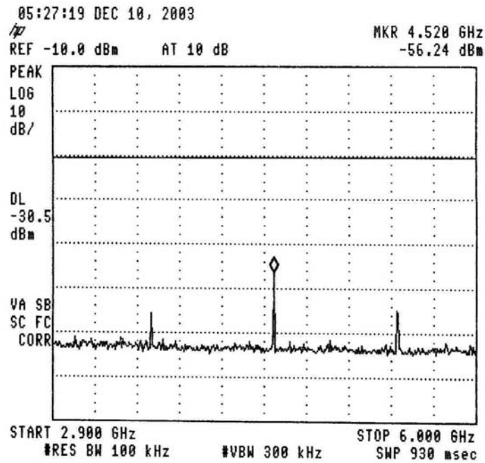
Figure 23.— 903.5 MHz
