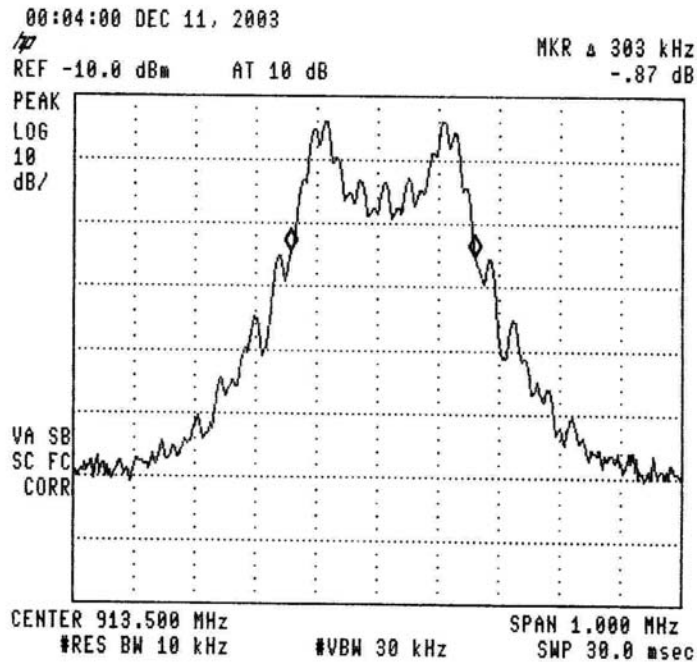
Figure 35 — 913.5 MHz
