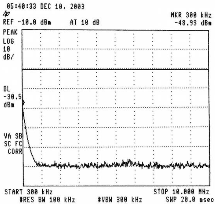
Figure 20.— 903.5 MHz
