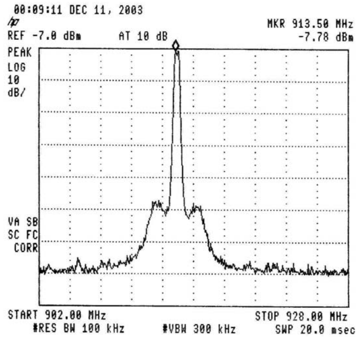
Figure 25.— 913.5 MHz
