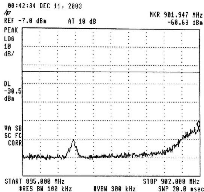
Figure 38 — 903.5 MHz
