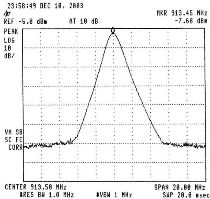
Figure 15.— 913.5 MHz
