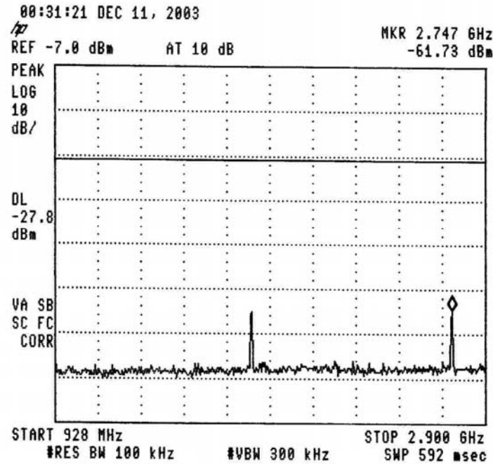
Figure 29.— 913.5 MHz
