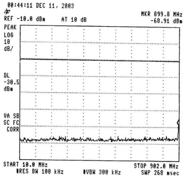
Figure 21.— 903.5 MHz
