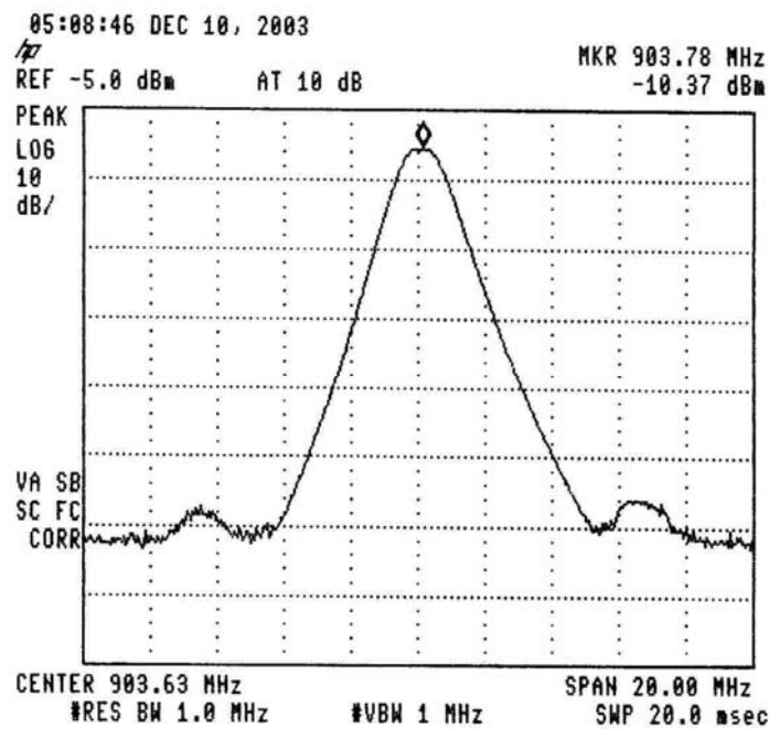
Figure 14.— 903.5 MHz
