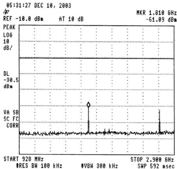
Figure 22.— 903.5 MHz
