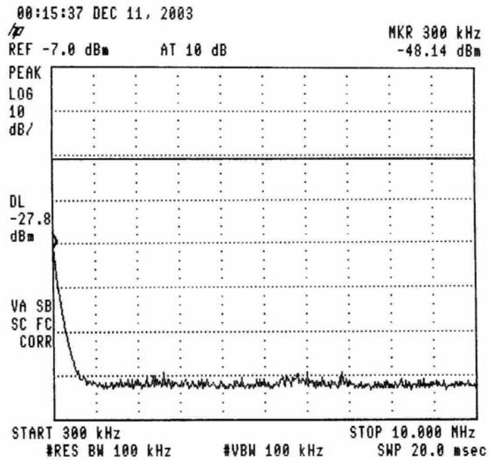
Figure 27.— 913.5 MHz
