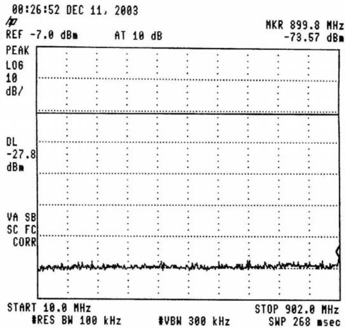
Figure 28.— 913.5 MHz
