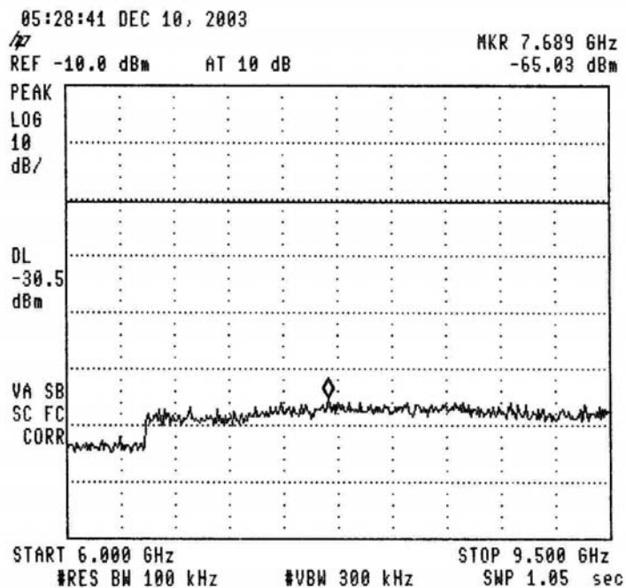
Figure 24.— 903.5 MHz
