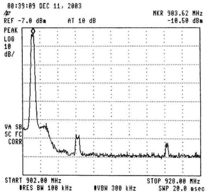
Figure 18.— 903.5 MHz
