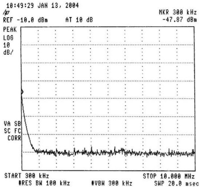
Figure 20.— 903.5 MHz
