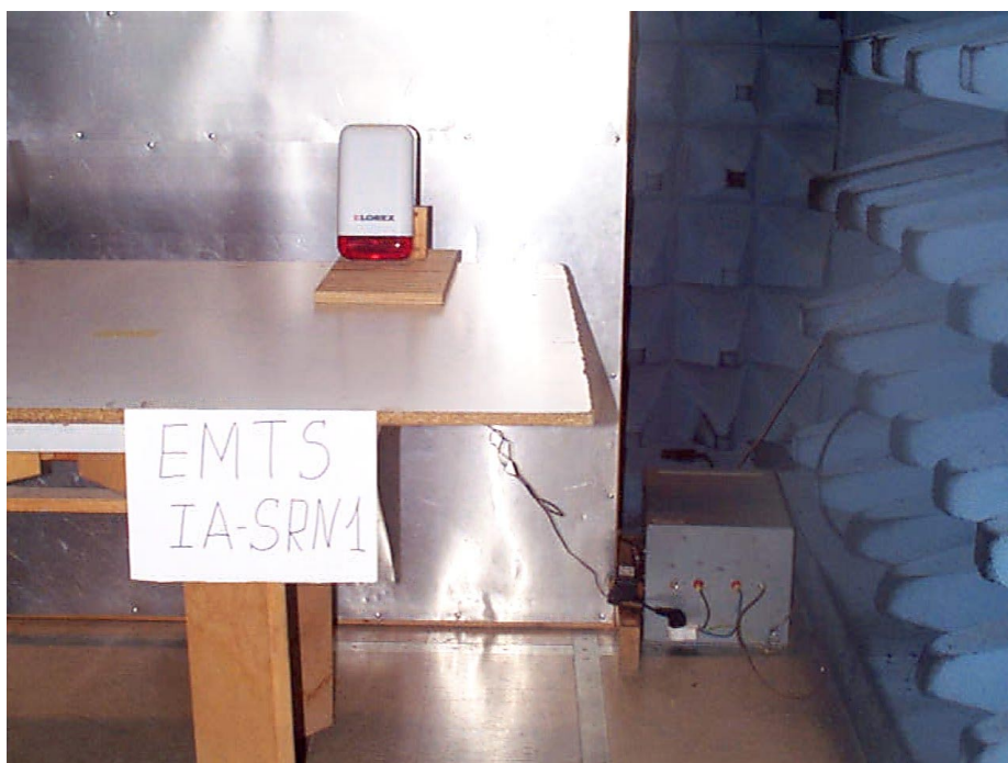
Figure 1. Conducted Emission Test.
