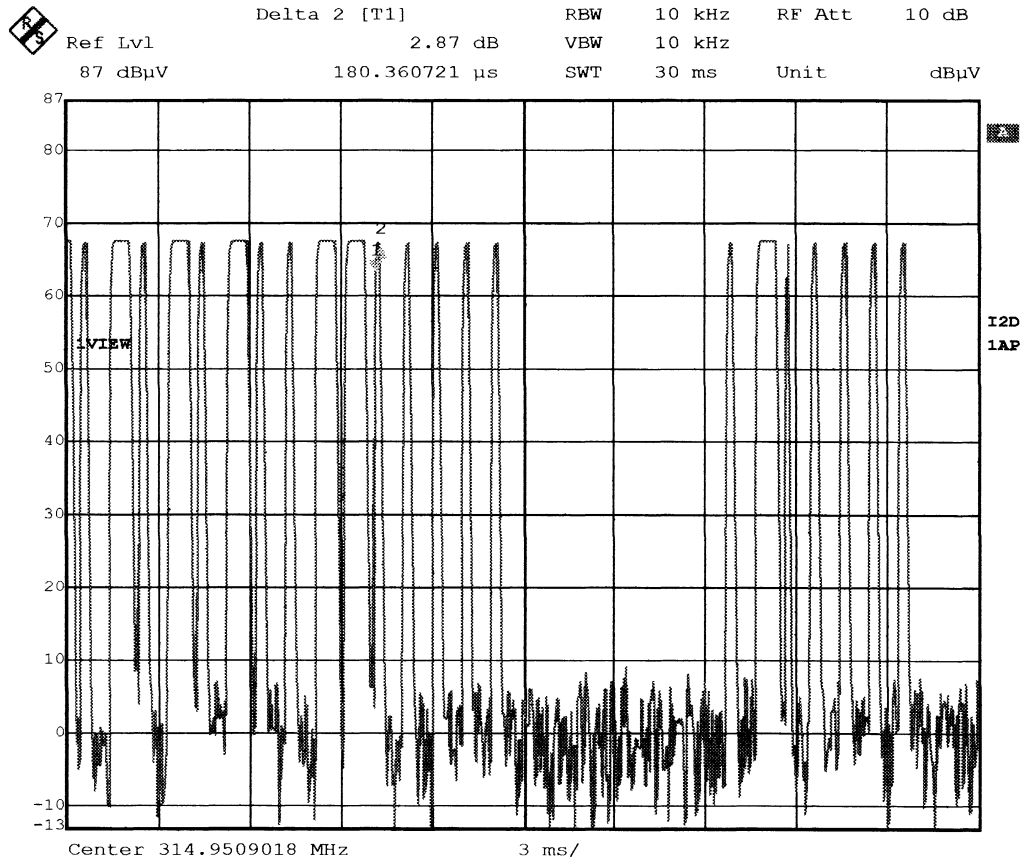
Figure C [Short Pulse]
