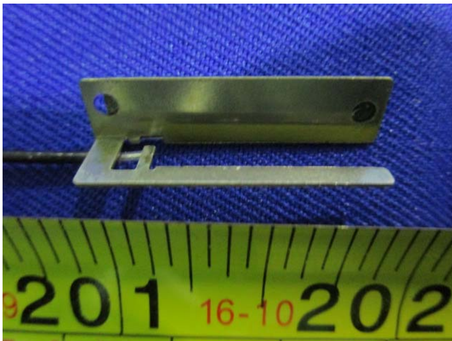
EUT –Antenna View (ThinkYard T000803)
