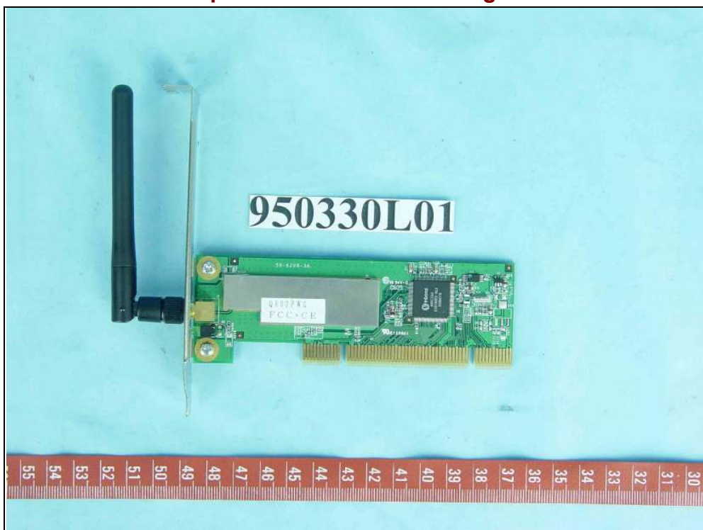
Dipole antenna with 2.5dBi gain
