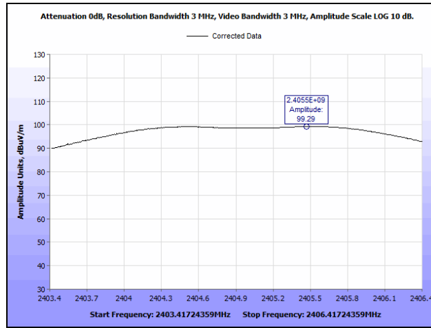
Plot 13. Peak Power Output, Low Channel
