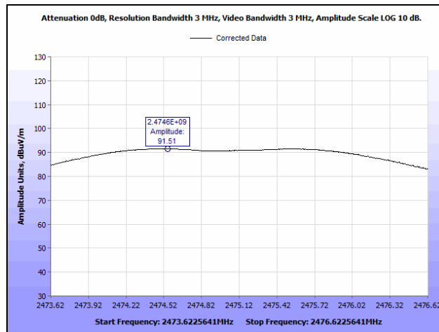
Plot 15. Peak Power Output, High Channel
