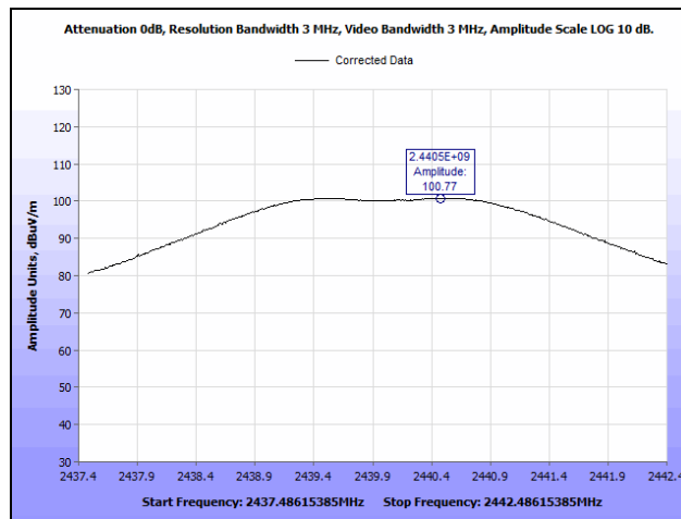
Plot 14. Peak Power Output, Mid Channel
