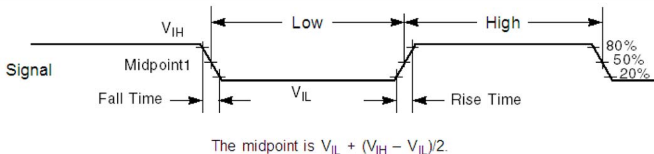
Figure 2. Input signal measurement reference
