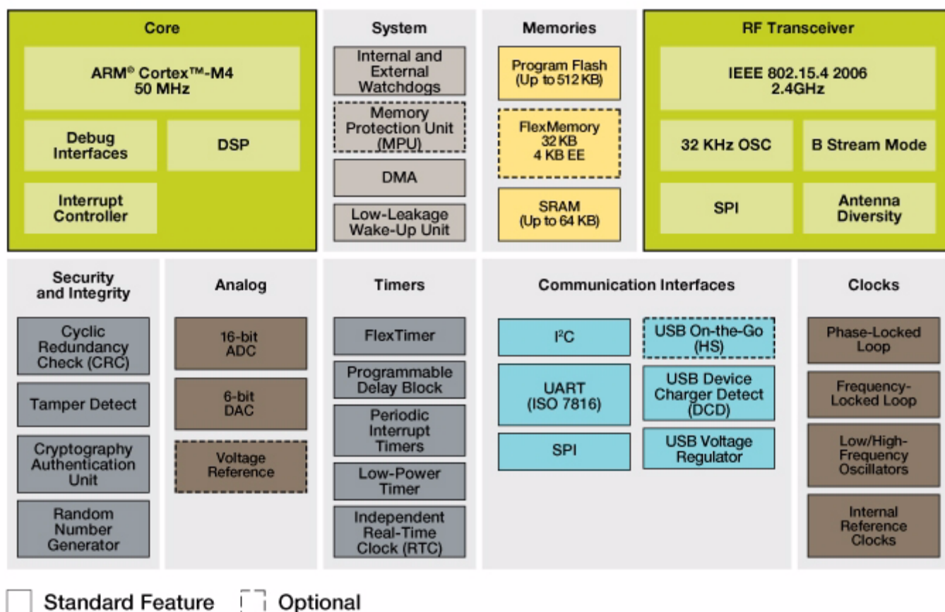
Figure 1. MKW2xDxxxV simplified block diagram
