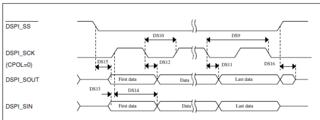
Figure 17. DSPI classic SPI timing — slave mode
