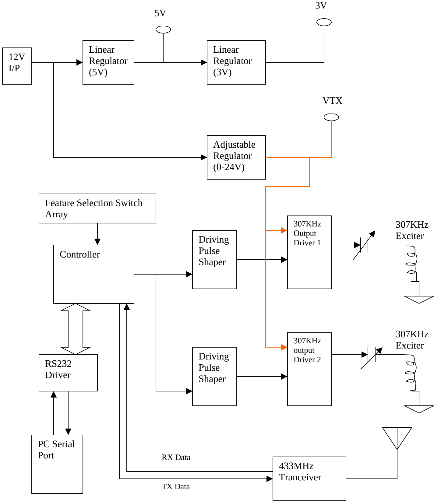
PTR Functional Block Diagram
