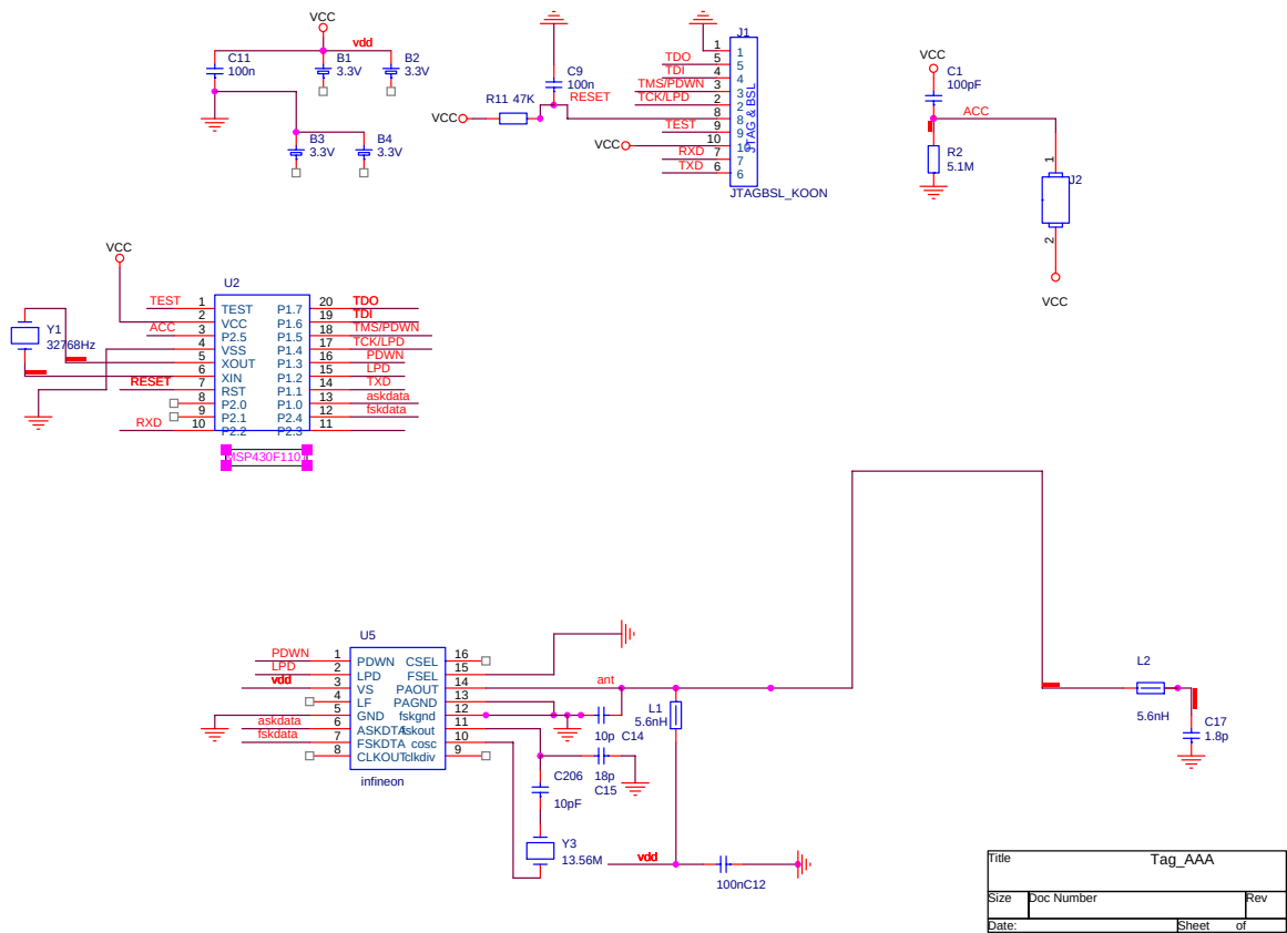
Figure 1: Tag_AAA schematic
