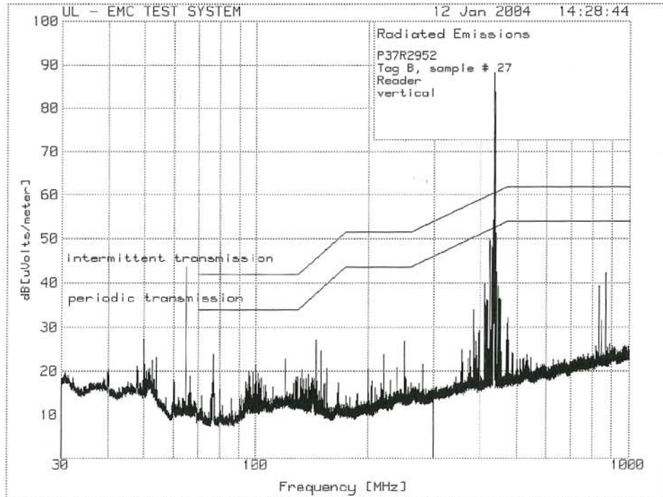
Radiated Emissions, 30 – 1000 MHz vertical peak prescan, Reader &amp; Tag B
