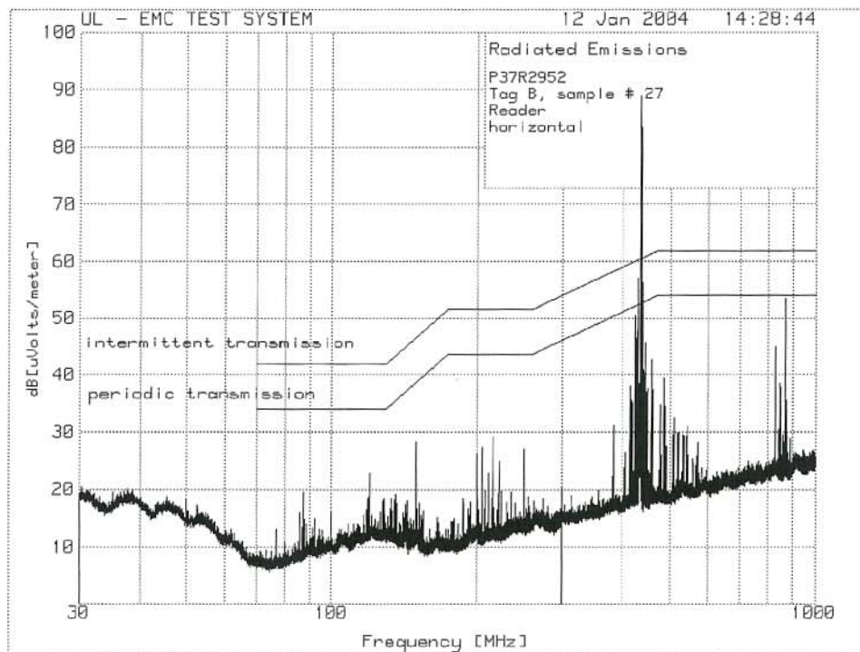
Radiated Emissions, 30 – 1000 MHz horizontal peak prescan, Reader &amp; Tag B
