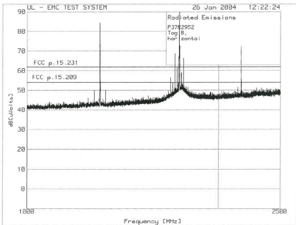
Radiated Emissions, 1 – 2.5 GHz horizontal peak prescan. Tag B
