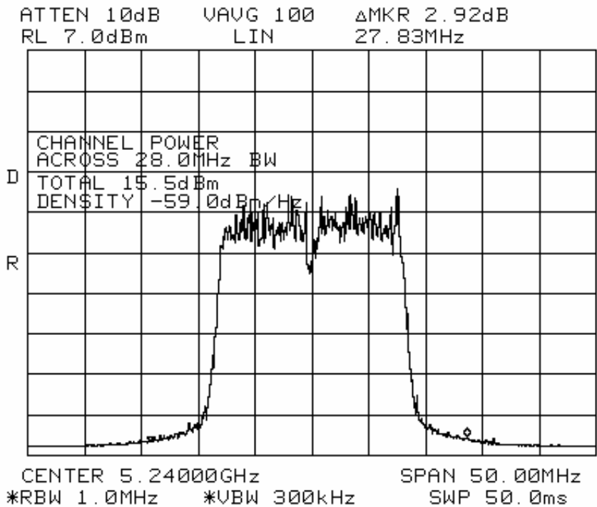
Pout @ 5240 MHz
