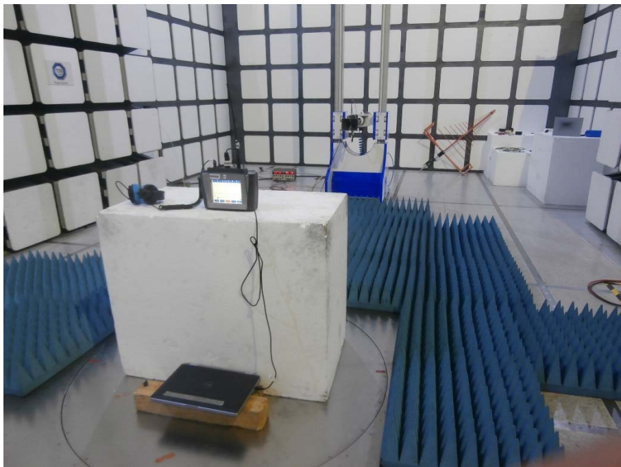
Radiated Emissions 1 GHz to 3 GHz
