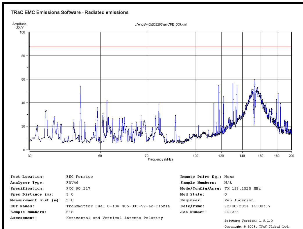
S18 TX 153.1MHz Radiated spurious emissions 30 MHz to 200 MHz
