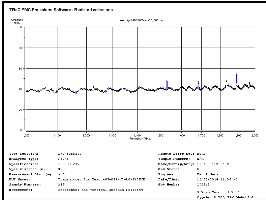
S15 TX 153.1MHz Radiated spurious emissions 1GHz to 2GHz
