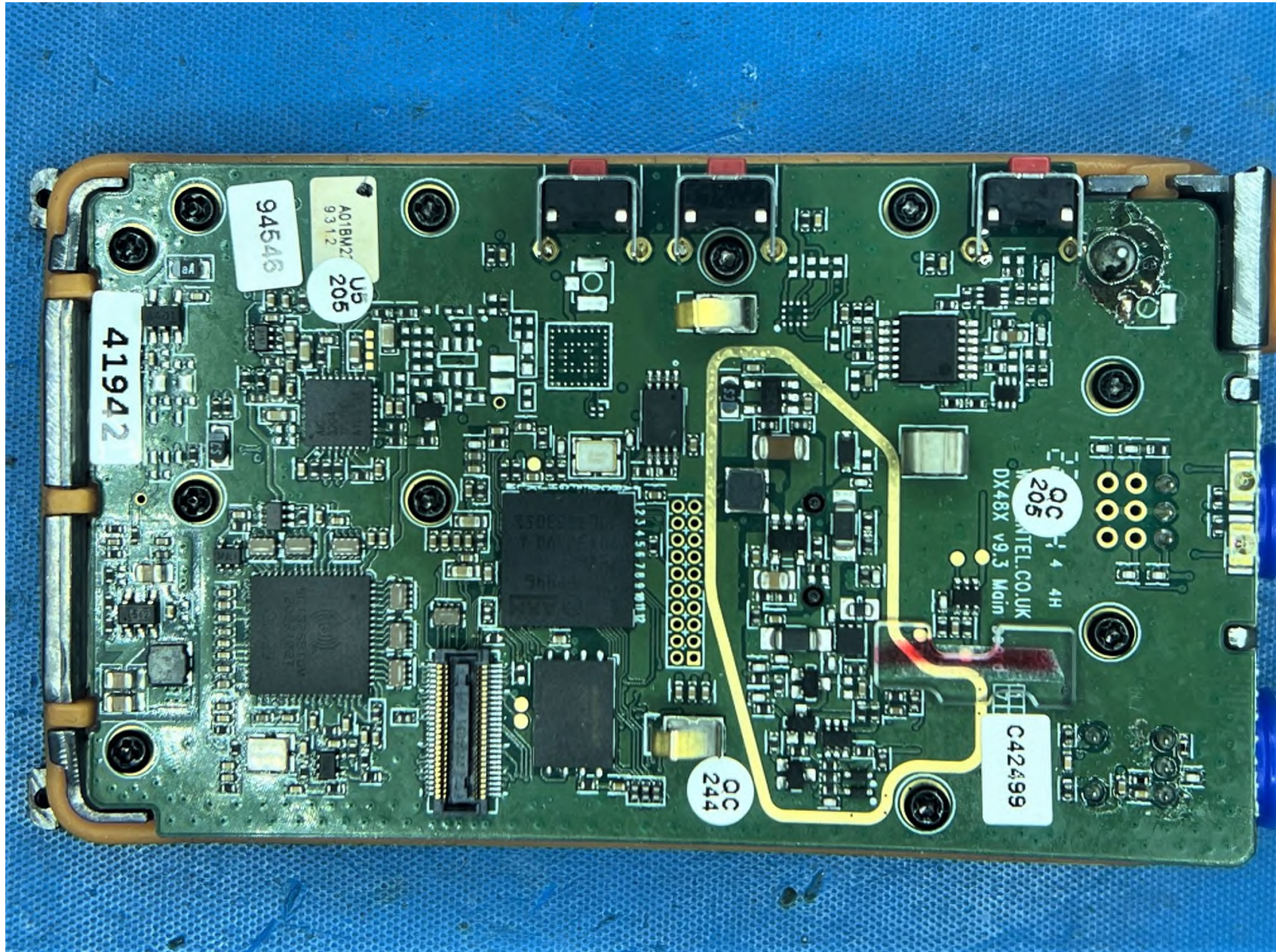
Main board top (close up)
