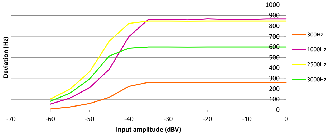
Modulation limiting 400.025 MHz Low Channel, Spacing 12.5 kHz
