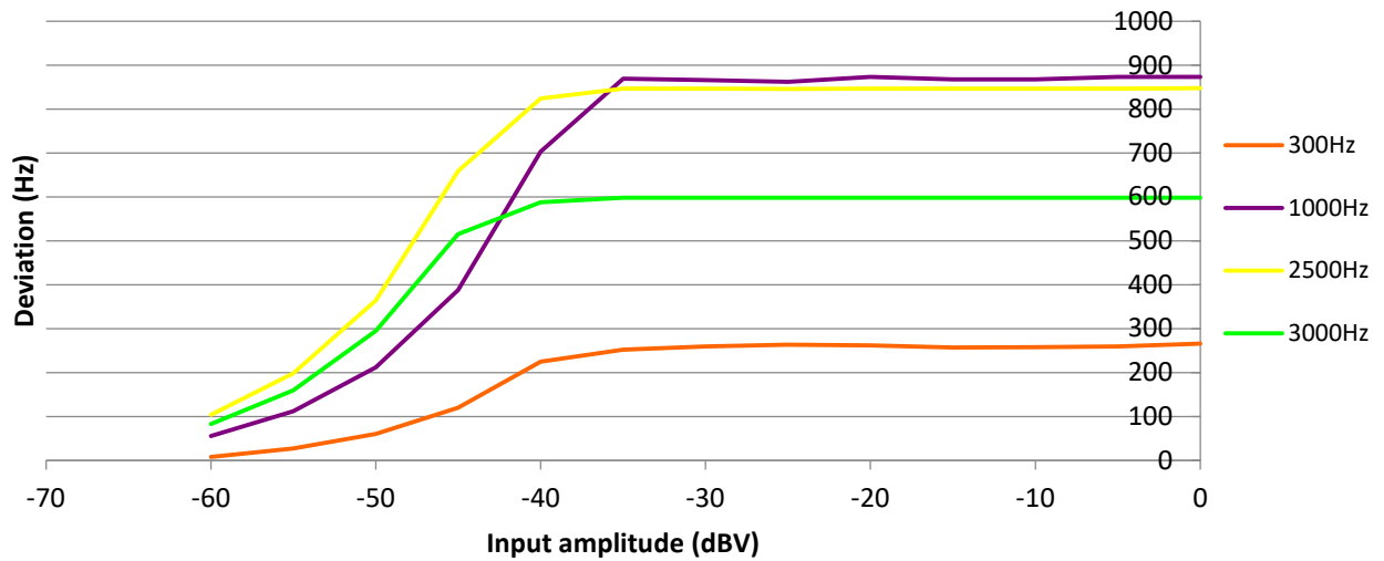
Modulation limiting 435 MHz Mid Channel, Spacing 12.5 kHz
