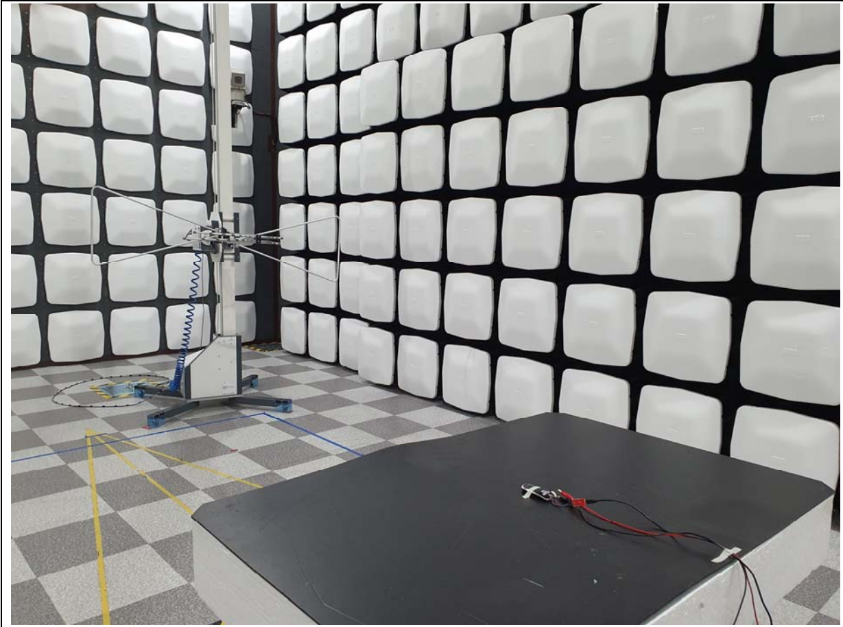
Below 1 GHz
